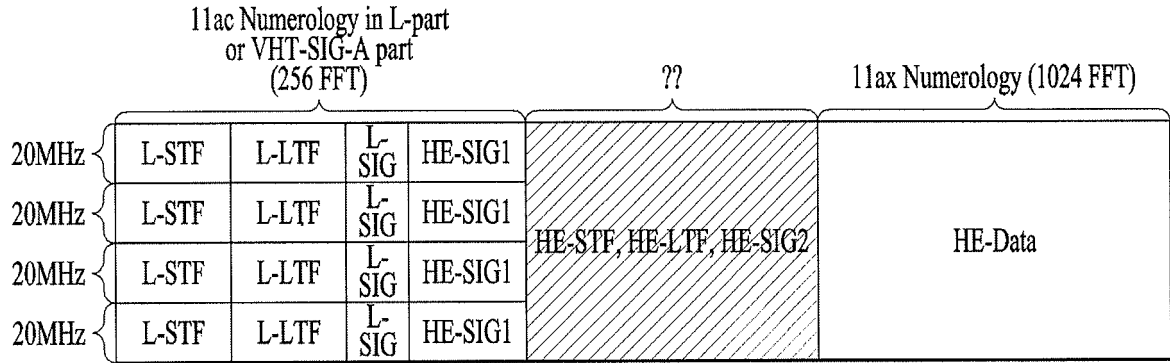
(a) HE PDU format
