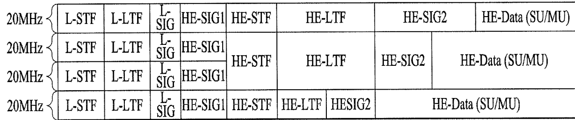
(b) HE PDU format
