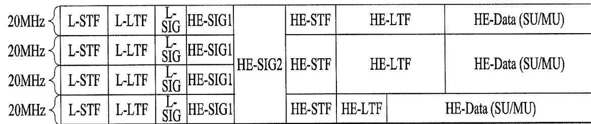
(c) HE PDU format
