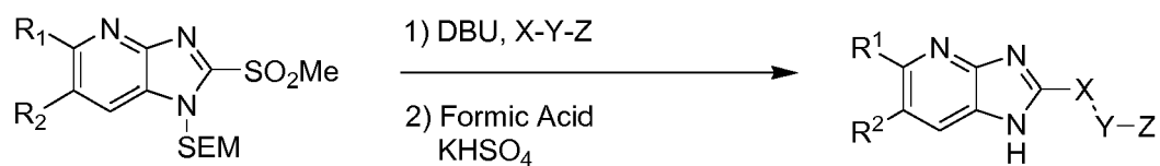
SCHEME 10
