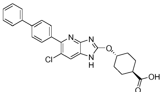
Trans-4-(((5-(biphenyl-4-yl)-6-chloro-1H-imidazo[4,5-b]pyridin-2-yl)oxy)cyclohexanecarboxylic acid
