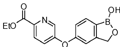
5-(1-Hydroxy-1,3-dihydro-benzo[c][1,2]oxaborol-5-yloxy)-pyridine-2-carboxylic acid ethyl ester
