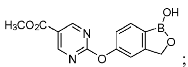
2-(1-Hydroxy-1,3-dihydro-benzo[c][1,2]oxaborol-5-yloxy)-thiazole-4-carboxylic acid methyl ester
