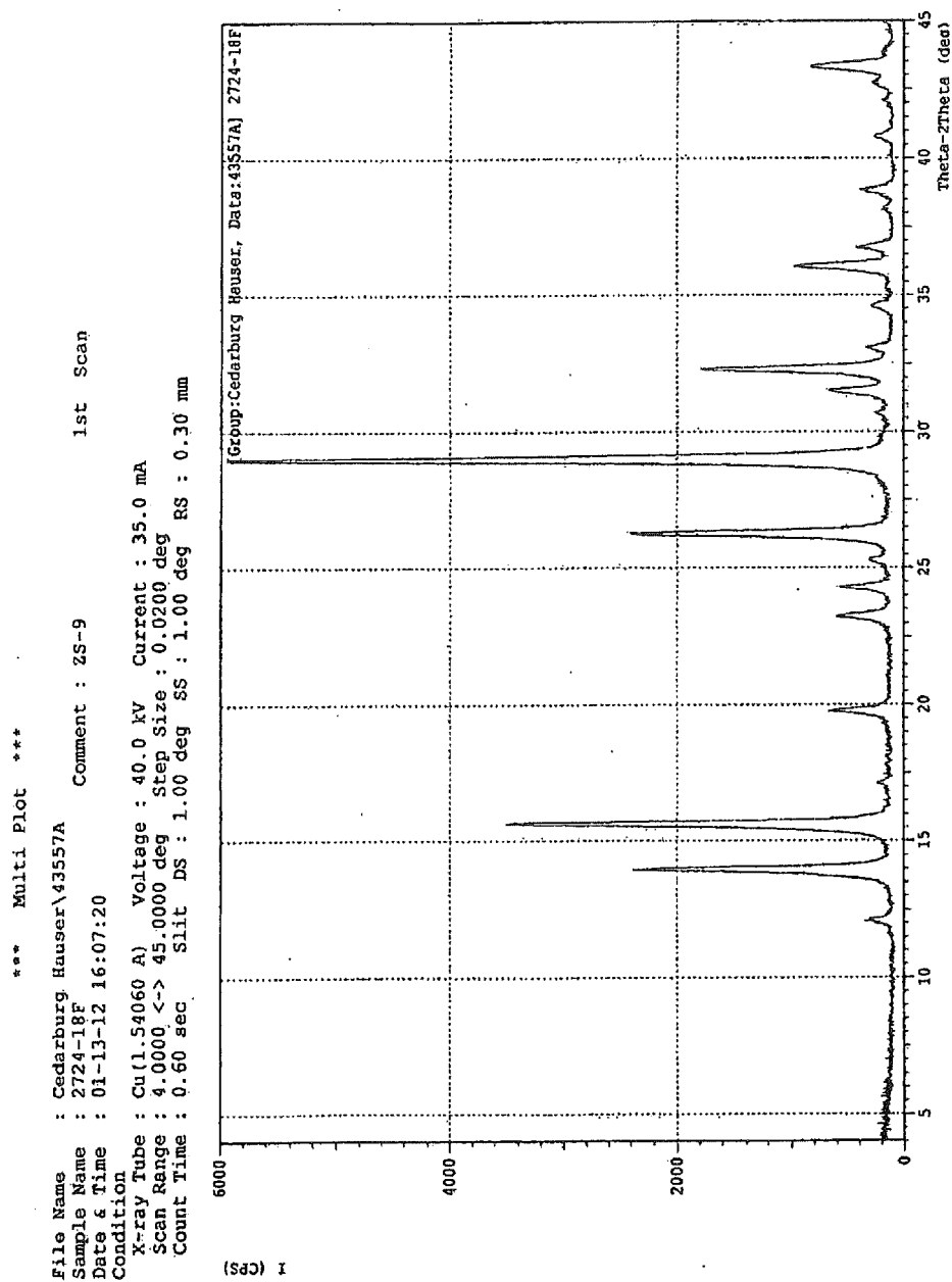
Fig. 12: XRD plot for ZS-9 prepared in accordance with Example 13.
