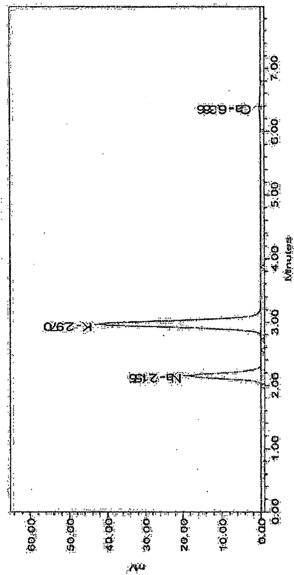
Fig. 16: Exemplary Sample Chromatogram.
