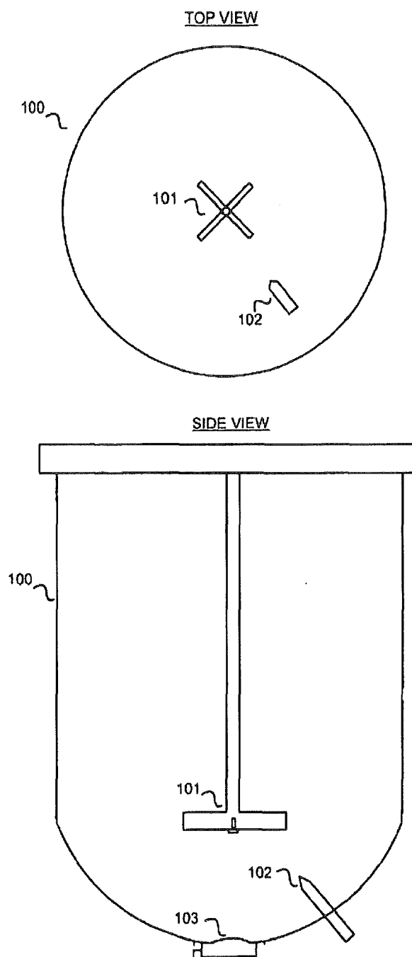
Fig. 17: 200-L reaction vessel with standard agitator arrangement.
