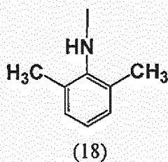
[Chemical Formula 33]
