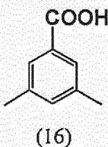
[Chemical Formula 8]
