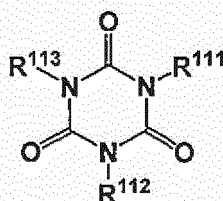
[Chemical Formula 35]
