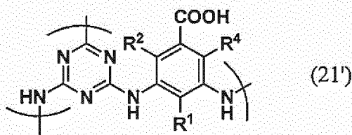
[Chemical Formula 30]
