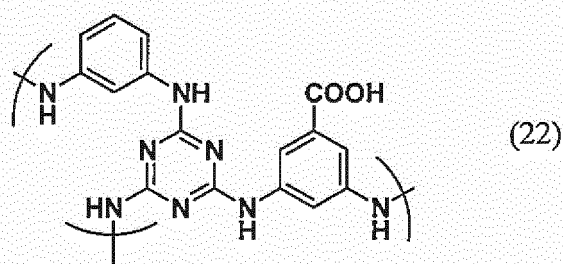
[Chemical Formula 28]
