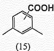
[Chemical Formula 7]
