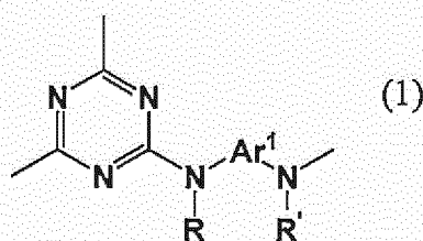
[Chemical Formula 11]
