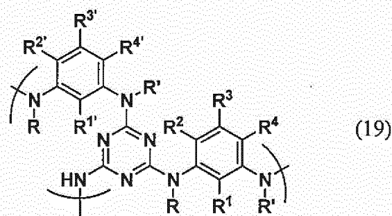
[Chemical Formula 24]
