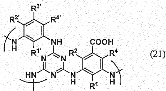
[Chemical Formula 26]
