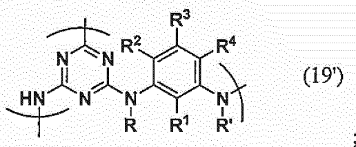
[Chemical Formula 28]
