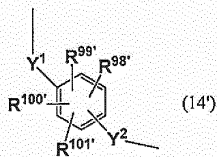
[Chemical Formula 6]
