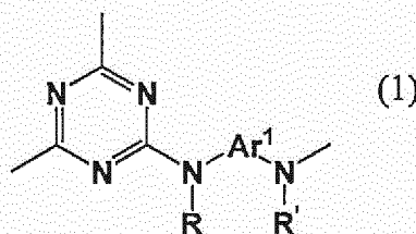
[Chemical Formula 1]
