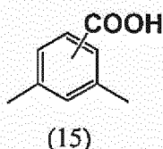
[Chemical Formula 7]
