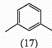
[Chemical Formula 9]
