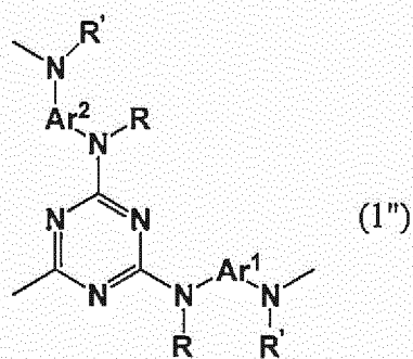
[Chemical Formula 23]
