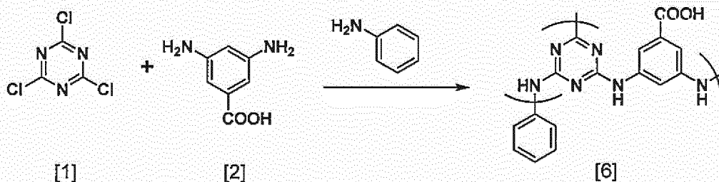
[Chemical Formula 37]
