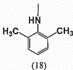
[Chemical Formula 10]
