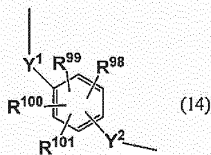
[Chemical Formula 13]
