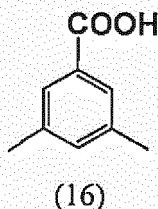
[Chemical Formula 8]
