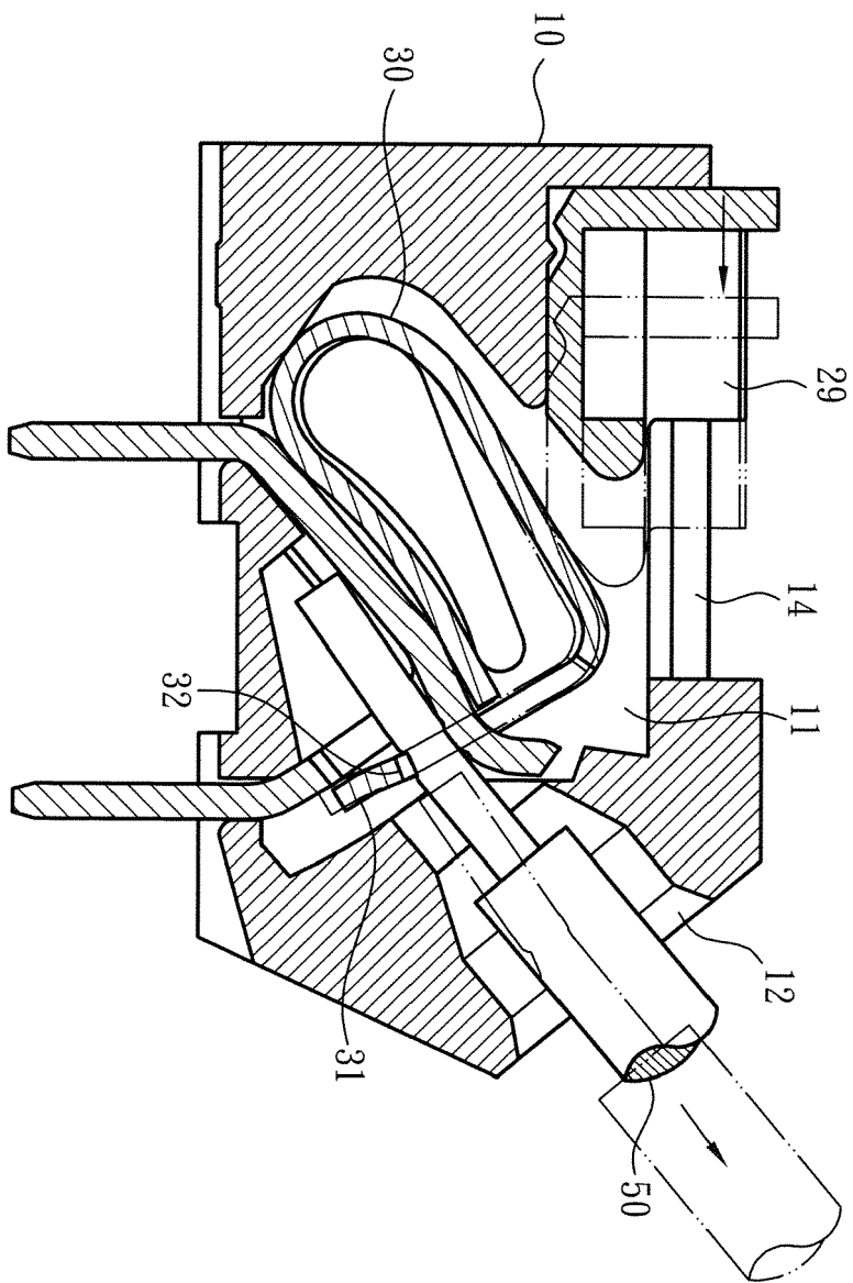
Fig. 3 PRIOR ART
