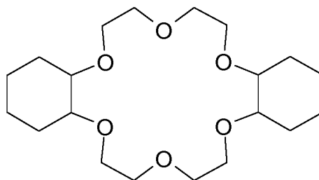
Dicyclohexano-18-crown-6
