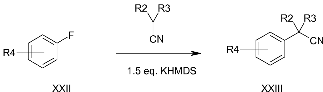
Scheme 8
