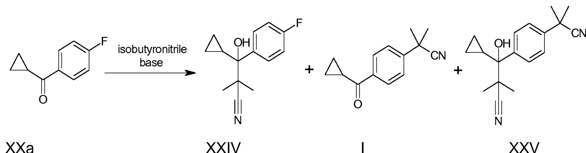
Scheme 9
