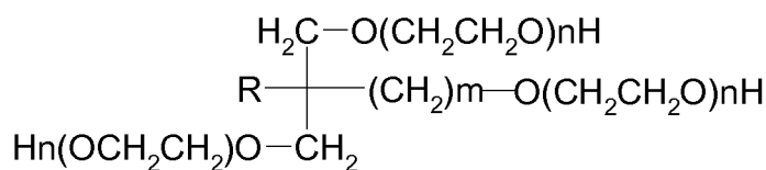
Formula XXXXVII
