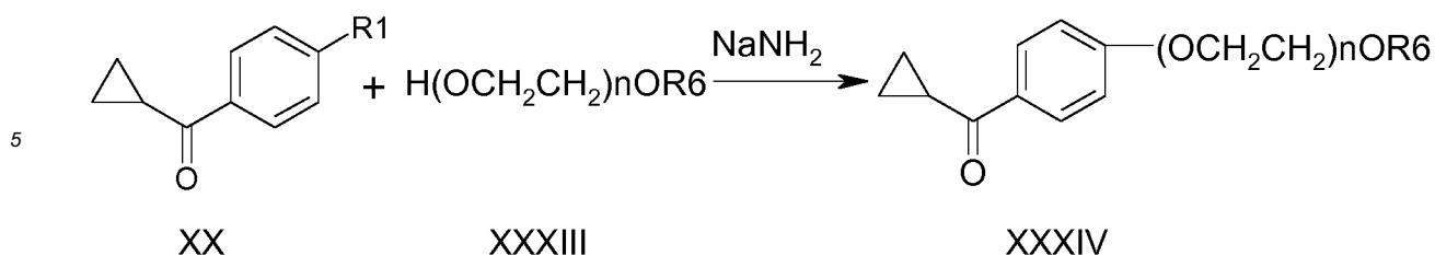
Scheme 11
