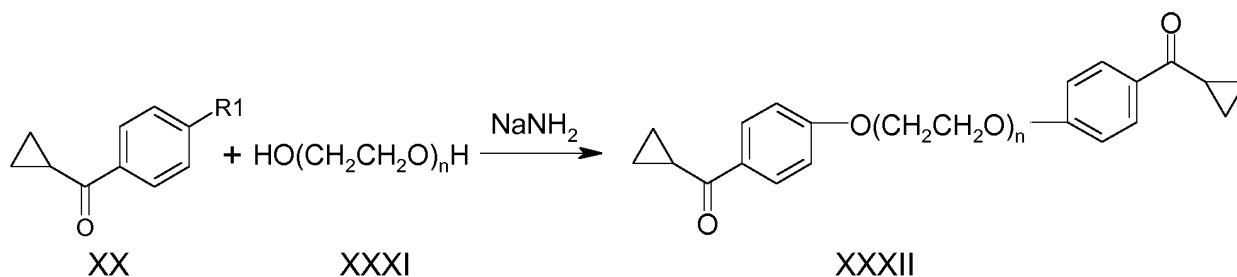
Scheme 10
