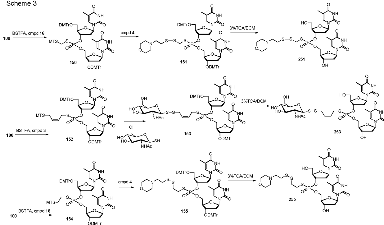
Scheme 3
