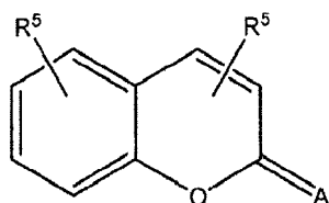
Scheme V
