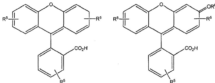
Scheme I
