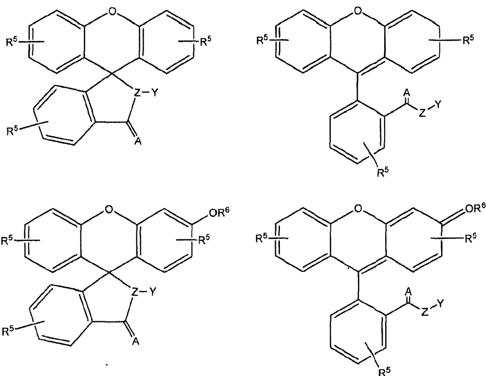
Scheme IV
