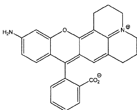
Scheme III
