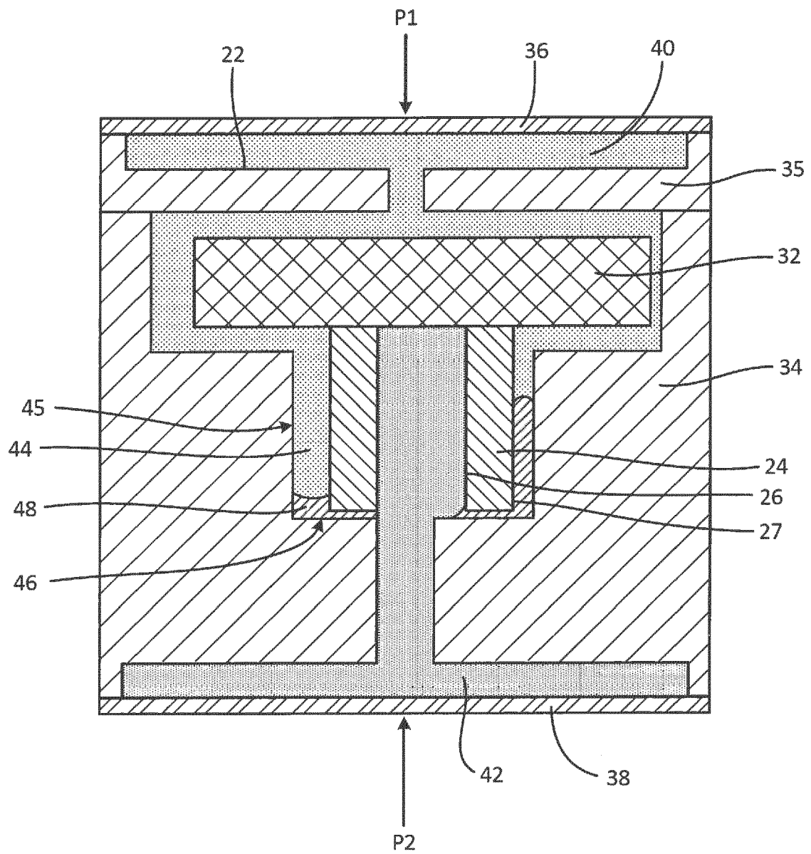
Fig. 3 Prior Art
