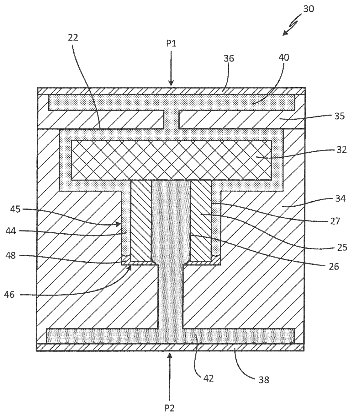
Fig. 2 Prior Art
