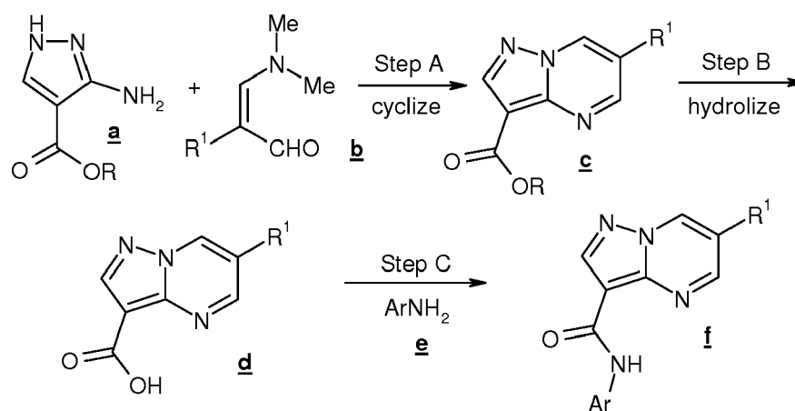
SCHEME A
