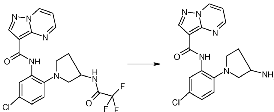
SCHEME 71
