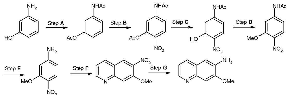
CHEME 29
