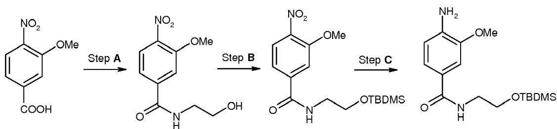
SCHEME 39
