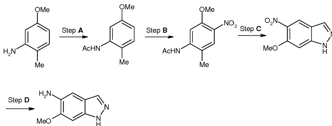
SCHEME 46
