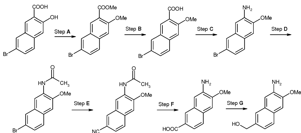
CHEME 26
