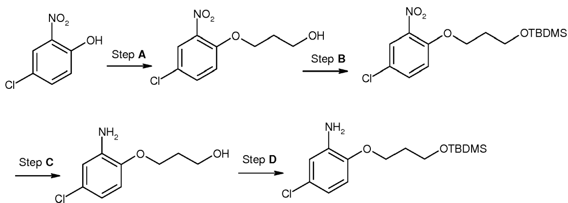
HEME 40
