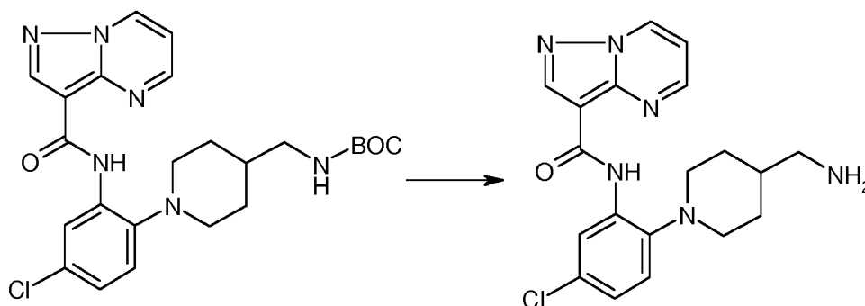
SCHEME 63
