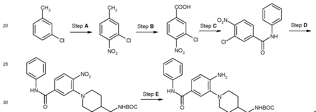
CHEME 37
