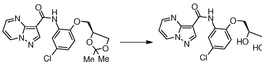
SCHEME 70
