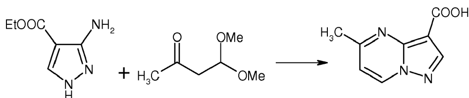
SCHEME 14
