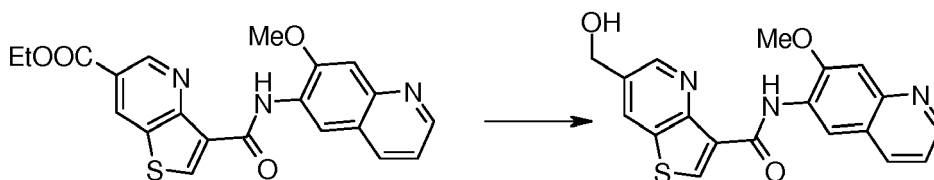
SCHEME 65
