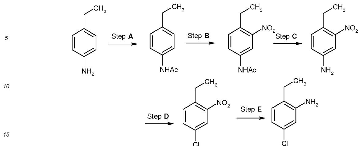
SCHEME 25
