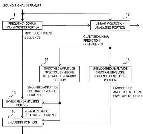
Fig. 1 CODES CORRESPONDING TO NORMALIZED MDCT COEFFICIENT SEQUENCE
