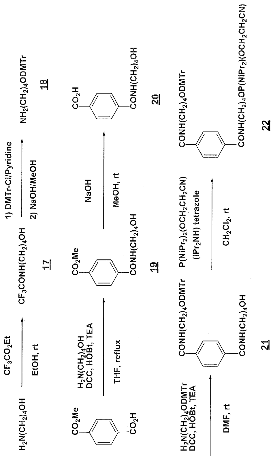
Scheme 7
