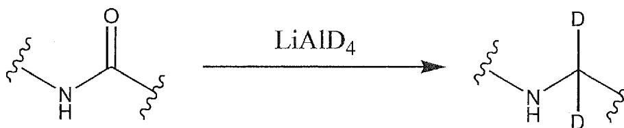
scheme 3a
