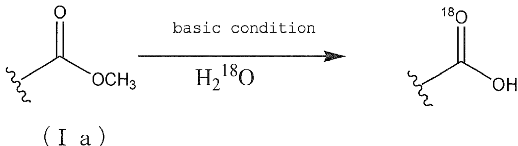
scheme 4a
