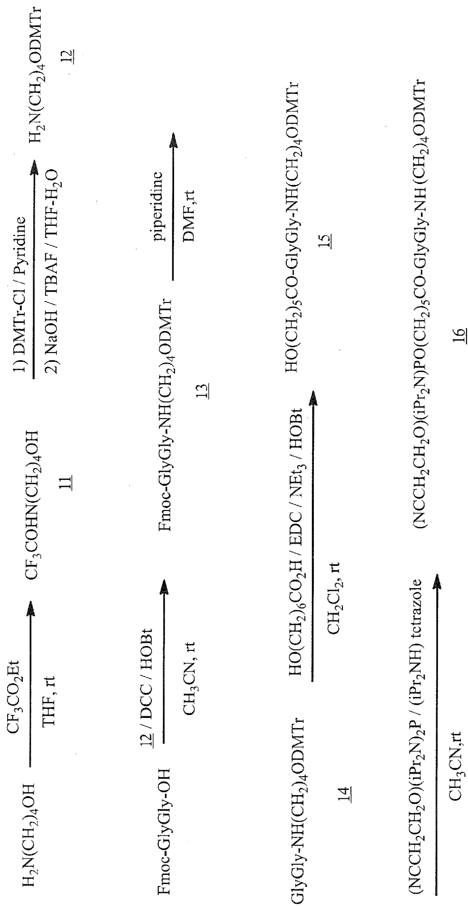
Scheme 6
