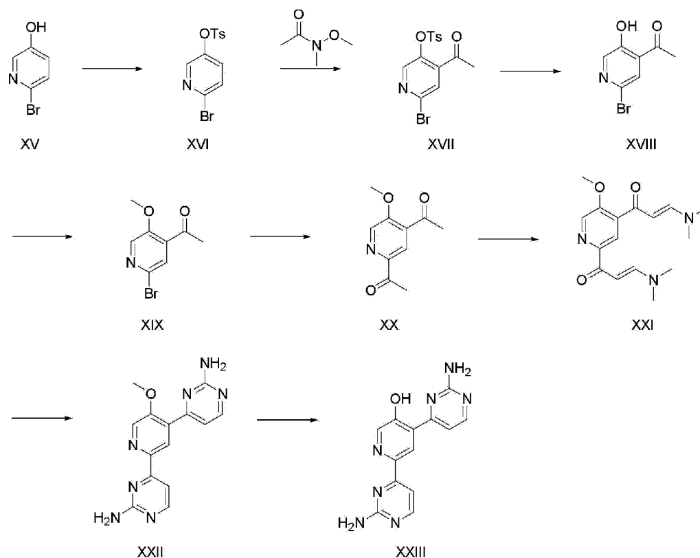
[Reaction Scheme 3]
