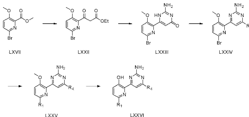
[Reaction Scheme 10]
