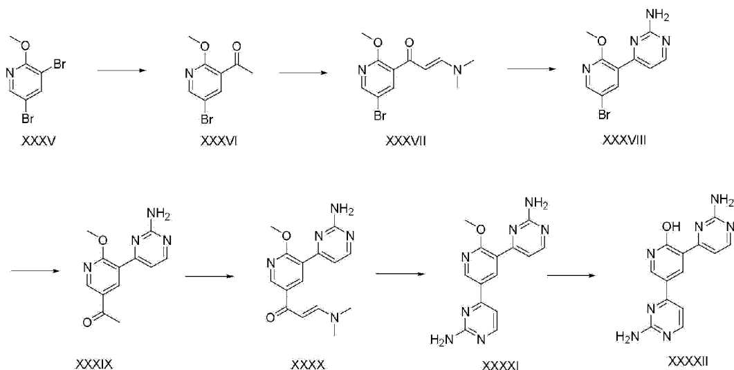
[Reaction Scheme 6]
