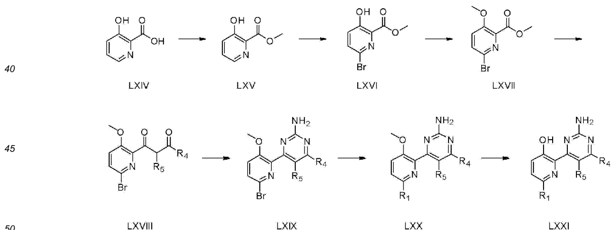
[Reaction Scheme 9]
