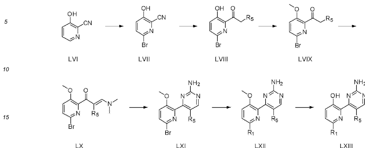
[Reaction Scheme 8]
