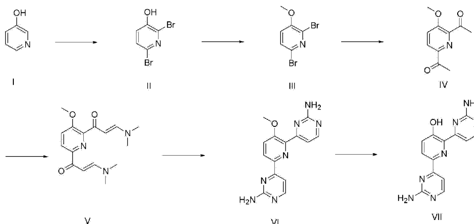
[Reaction Scheme 1]
