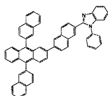
[Chemical Formula 282]
