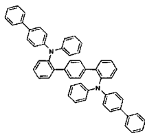
[Chemical Formula 342]
