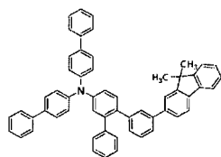
[Chemical Formula 46]
