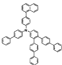
[Chemical Formula 165]
