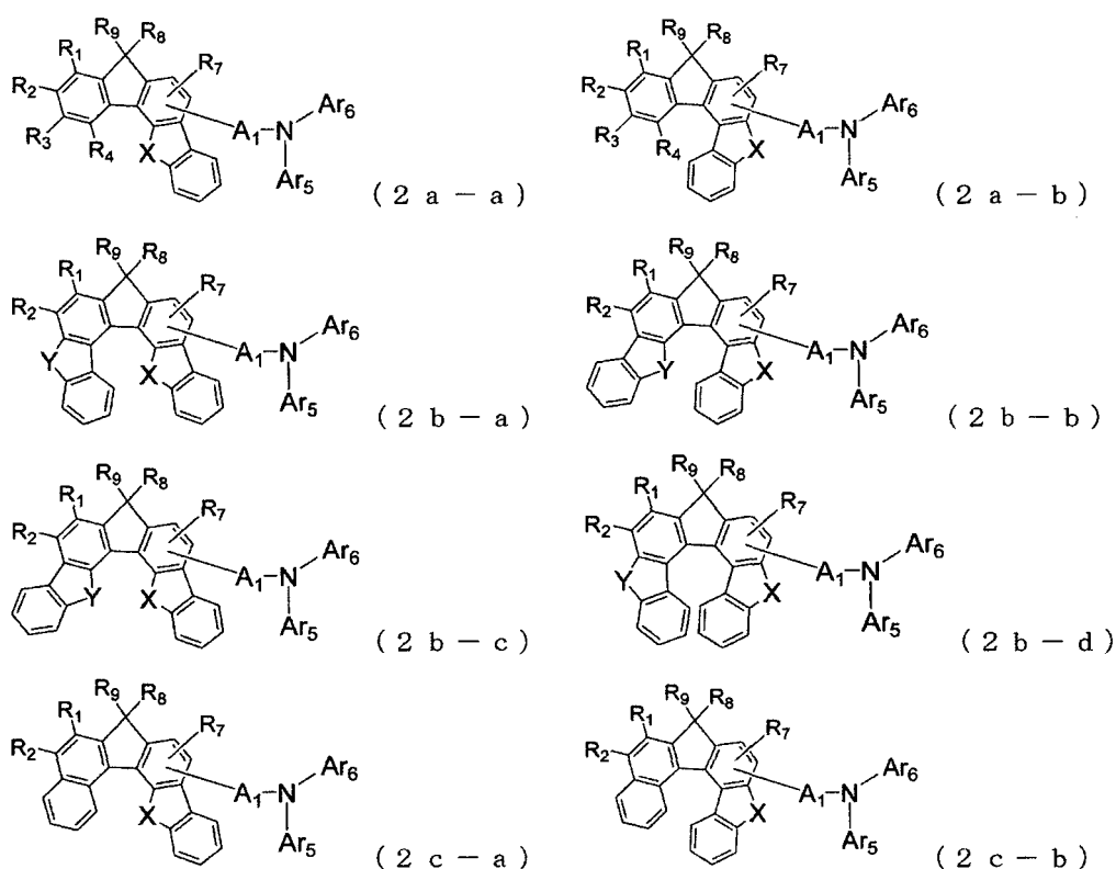
[Chemical Formula 9]
