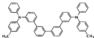
[Chemical Formula 351]
