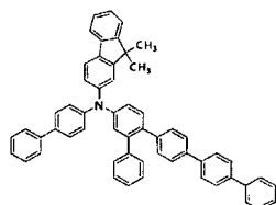
[Chemical Formula 82]
