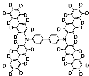
[Chemical Formula 335]
