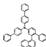
[Chemical Formula 111]
