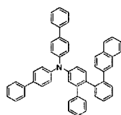
[Chemical Formula 44]
