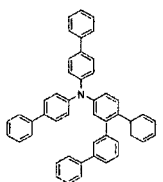
[Chemical Formula 116]
