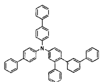
[Chemical Formula 30]
