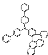
[Chemical Formula 114]
