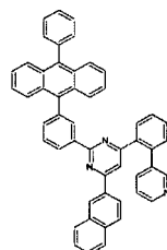
[Chemical Formula 291]
