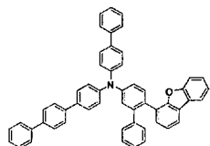
[Chemical Formula 97]
