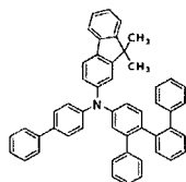
[Chemical Formula 187]
