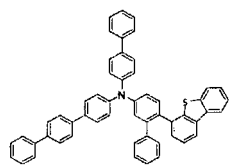
[Chemical Formula 98]
