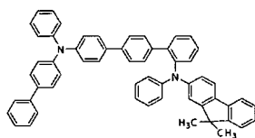
[Chemical Formula 344]
