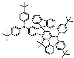
[Chemical Formula 236]
