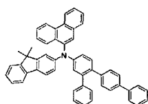
[Chemical Formula 224]
