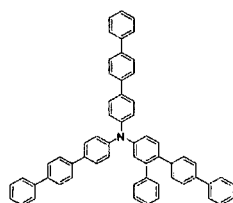
[Chemical Formula 105]
