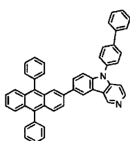
[Chemical Formula 256]
