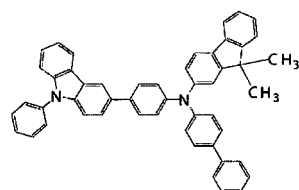
[Chemical Formula 356]
