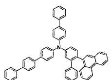
[Chemical Formula 92]
