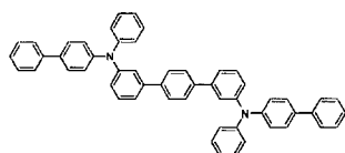
[Chemical Formula 341]
