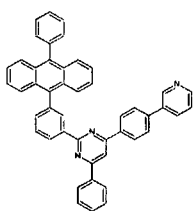
[Chemical Formula 297]
