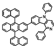
[Chemical Formula 251]
