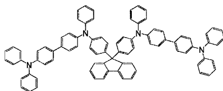
[Chemical Formula 369]
