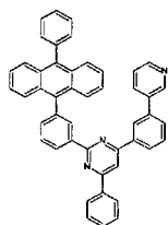
[Chemical Formula 284]
