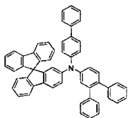
[Chemical Formula 197]
