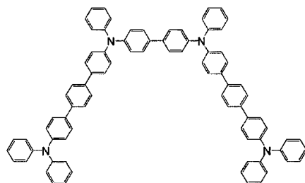
[Chemical Formula 359]
