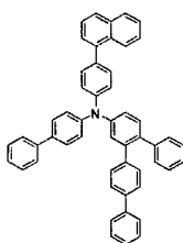
[Chemical Formula 164]
