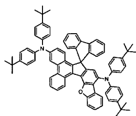
[Chemical Formula 228]
