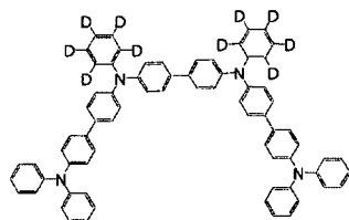
[Chemical Formula 370]
