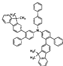
[Chemical Formula 146]
