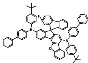
[Chemical Formula 232]
