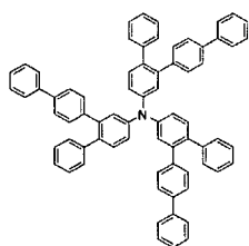
[Chemical Formula 158]
