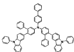
[Chemical Formula 127]
