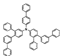
[Chemical Formula 124]
