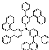
[Chemical Formula 157]
