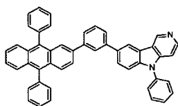
[Chemical Formula 262]
