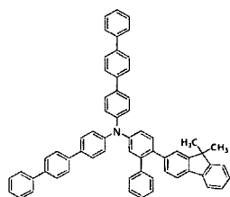
[Chemical Formula 102]
