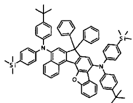
[Chemical Formula 243]
