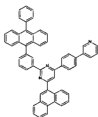
[Chemical Formula 303]
