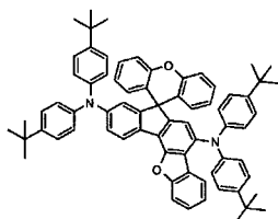
[Chemical Formula 406]
