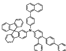
[Chemical Formula 206]
