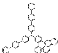
[Chemical Formula 104]
