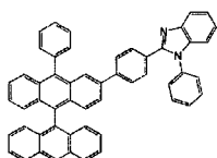
[Chemical Formula 277]
