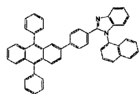
[Chemical Formula 272]
