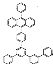
[Chemical Formula 288]
