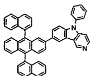
[Chemical Formula 255]
