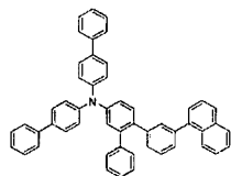
[Chemical Formula 40]
