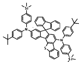
[Chemical Formula 234]
