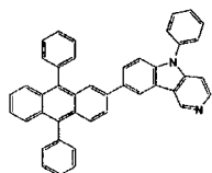
[Chemical Formula 418]
