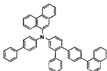
[Chemical Formula 216]
