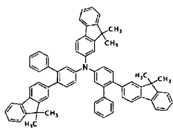
[Chemical Formula 140]
