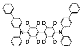
[Chemical Formula 329]
