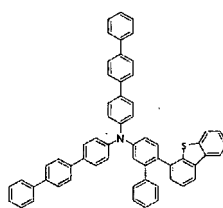
[Chemical Formula 110]
