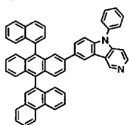
[Chemical Formula 255]
