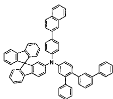
[Chemical Formula 211]
