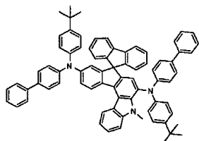
[Chemical Formula 237]
