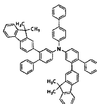
[Chemical Formula 143]
