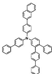
[Chemical Formula 422]
