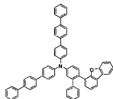
[Chemical Formula 109]
