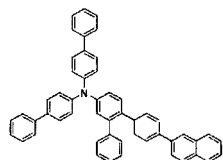
[Chemical Formula 42]
