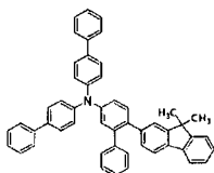
[Chemical Formula 28]
