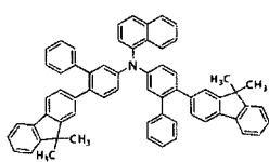
[Chemical Formula 136]
