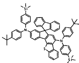
[Chemical Formula 409]
