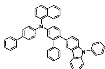
[Chemical Formula 72]
