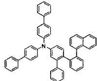
[Chemical Formula 41]
