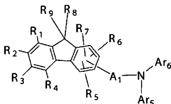
[Chemical Formula 2]
