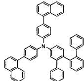
[Chemical Formula 175]
