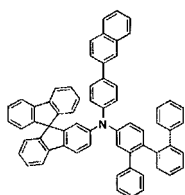
[Chemical Formula 211]
