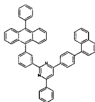
[Chemical Formula 286]
