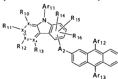
[Chemical Formula 6]
