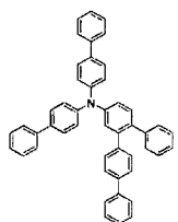
[Chemical Formula 115]
