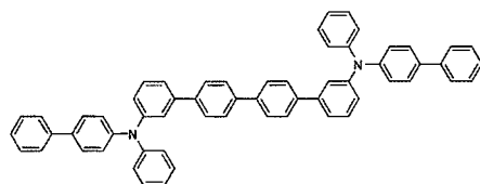
[Chemical Formula 347]
