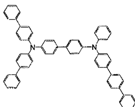
[Chemical Formula 317]
