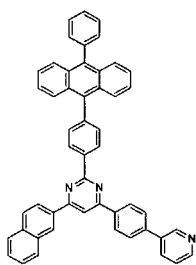
[Chemical Formula 310]
