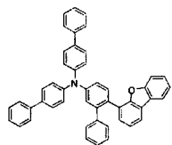
[Chemical Formula 38]
