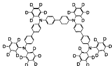
[Chemical Formula 371]
