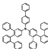
[Chemical Formula 125]
