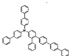
[Chemical Formula 34]
