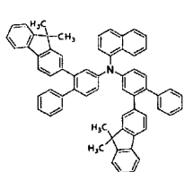
[Chemical Formula 150]
