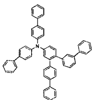
[Chemical Formula 160]
