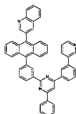
[Chemical Formula 292]
