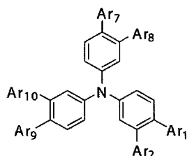
[Chemical Formula 4]
