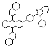
[Chemical Formula 269]
