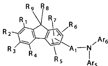
[Chemical Formula 2]
