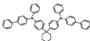
[Chemical Formula 319]
