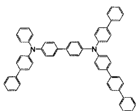
[Chemical Formula 318]
