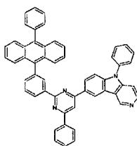
[Chemical Formula 305]
