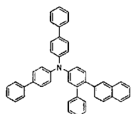
[Chemical Formula 32]
