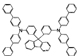
[Chemical Formula 322]
