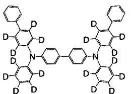
[Chemical Formula 331]
