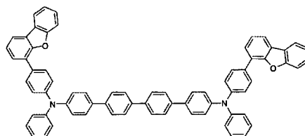
[Chemical Formula 353]
