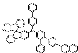
[Chemical Formula 203]
