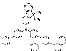
[Chemical Formula 189]
