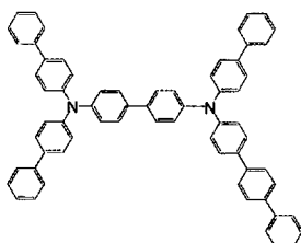
[Chemical Formula 316]
