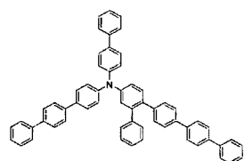
[Chemical Formula 94]
