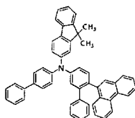
[Chemical Formula 80]
