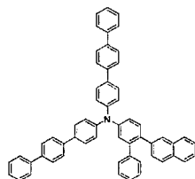
[Chemical Formula 102]
