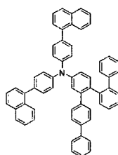
[Chemical Formula 179]
