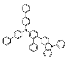
[Chemical Formula 35]
