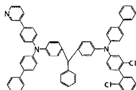
[Chemical Formula 324]
