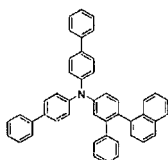
[Chemical Formula 27]
