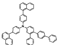
[Chemical Formula 173]
