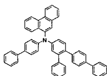
[Chemical Formula 213]
