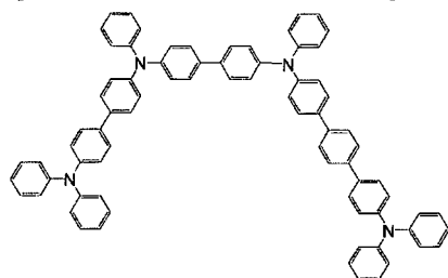
[Chemical Formula 361]
