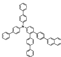
[Chemical Formula 163]
