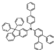
[Chemical Formula 190]
