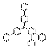
[Chemical Formula 415]
