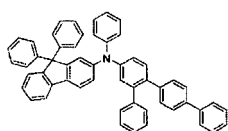
[Chemical Formula 194]
