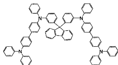
[Chemical Formula 366]
