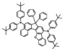
[Chemical Formula 240]
