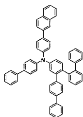
[Chemical Formula 171]
