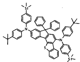
[Chemical Formula 244]
