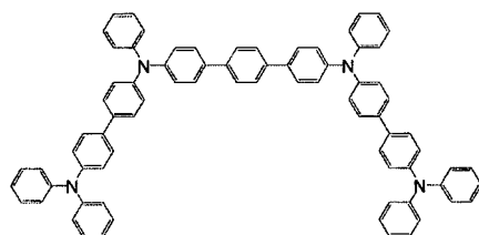
[Chemical Formula 358]
