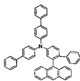
[Chemical Formula 113]
