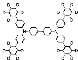
[Chemical Formula 333]
