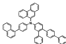
[Chemical Formula 218]
