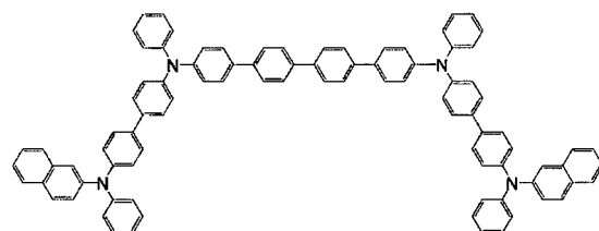
[Chemical Formula 364]
