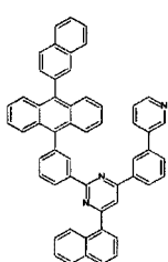
[Chemical Formula 297]
