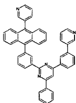
[Chemical Formula 293]
