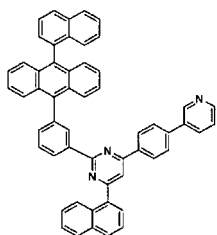
[Chemical Formula 313]
