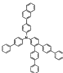
[Chemical Formula 169]
