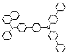
[Chemical Formula 326]
