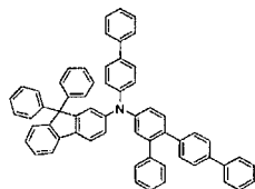
[Chemical Formula 191]
