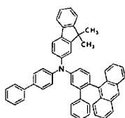
[Chemical Formula 79]
