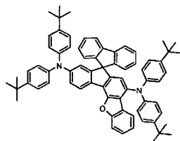
[Chemical Formula 227]
