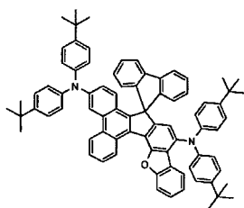
[Chemical Formula 403]
