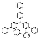
[Chemical Formula 117]
