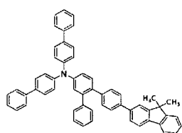
[Chemical Formula 45]
