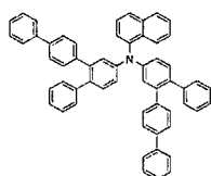
[Chemical Formula 145]
