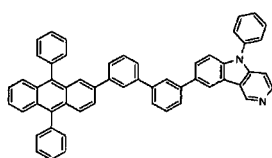
[Chemical Formula 265]
