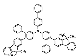
[Chemical Formula 122]
