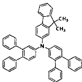
[Chemical Formula 138]
