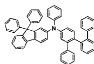
[Chemical Formula 196]
