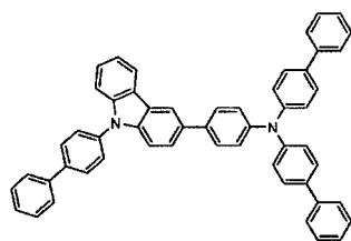
[Chemical Formula 356]
