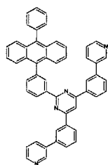
[Chemical Formula 299]
