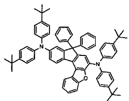
[Chemical Formula 241]
