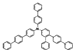
[Chemical Formula 93]
