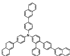
[Chemical Formula 184]
