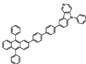
[Chemical Formula 265]
