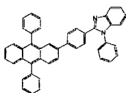
[Chemical Formula 269]
