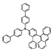
[Chemical Formula 33]
