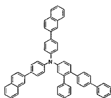
[Chemical Formula 180]
