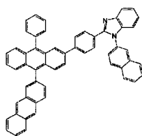
[Chemical Formula 279]
