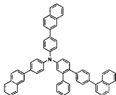
[Chemical Formula 424]
