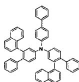
[Chemical Formula 142]
