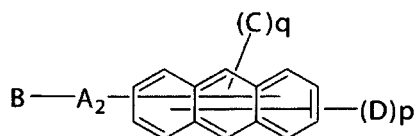
[Chemical Formula 5]
