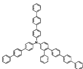
[Chemical Formula 106]
