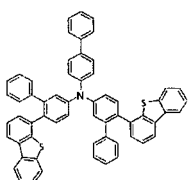
[Chemical Formula 129]
