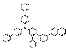
[Chemical Formula 43]
