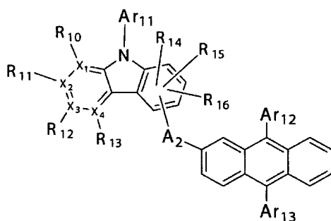
[Chemical Formula 6]
