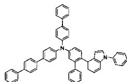
[Chemical Formula 95]
