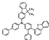
[Chemical Formula 86]
