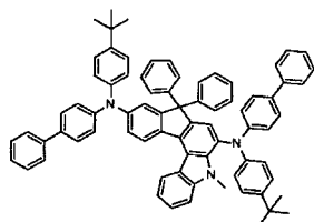
[Chemical Formula 247]
