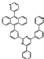
[Chemical Formula 294]
