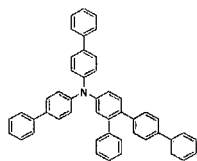
[Chemical Formula 421]
