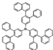
[Chemical Formula 155]
