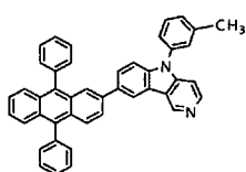
[Chemical Formula 260]
