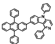
[Chemical Formula 250]
