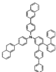
[Chemical Formula 185]
