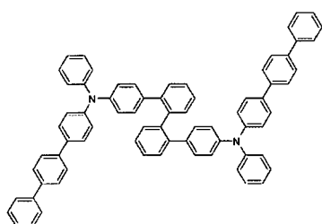
[Chemical Formula 348]
