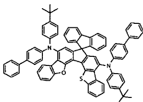
[Chemical Formula 410]
