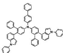
[Chemical Formula 127]
