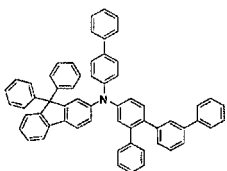
[Chemical Formula 391]
