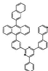
[Chemical Formula 285]
