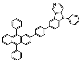
[Chemical Formula 261]
