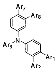
[Chemical Formula 3]
