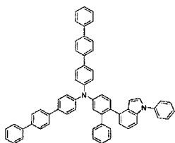
[Chemical Formula 107]
