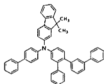
[Chemical Formula 186]
