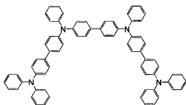
[Chemical Formula 357]
