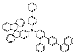
[Chemical Formula 202]
