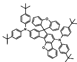
[Chemical Formula 231]
