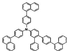
[Chemical Formula 176]
