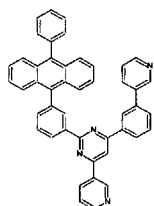
[Chemical Formula 301]
