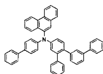
[Chemical Formula 214]
