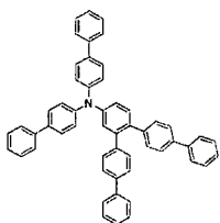
[Chemical Formula 159]
