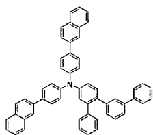
[Chemical Formula 181]
