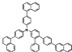
[Chemical Formula 177]
