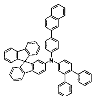
[Chemical Formula 208]
