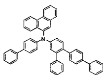
[Chemical Formula 399]
