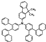
[Chemical Formula 139]
