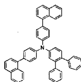
[Chemical Formula 172]
