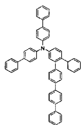
[Chemical Formula 118]
