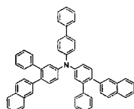
[Chemical Formula 122]
