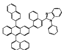
[Chemical Formula 279]
