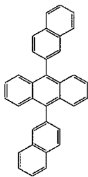
[Chemical Formula 417]
