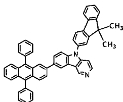
[Chemical Formula 260]
