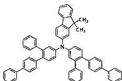
[Chemical Formula 141]
