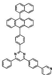
[Chemical Formula 313]
