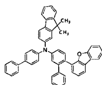
[Chemical Formula 86]
