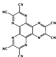
[Chemical Formula 413]
