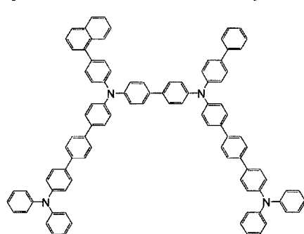
[Chemical Formula 362]
