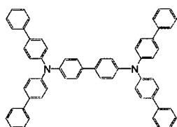
[Chemical Formula 414]
