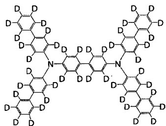
[Chemical Formula 336]
