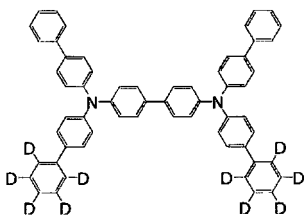
[Chemical Formula 332]
