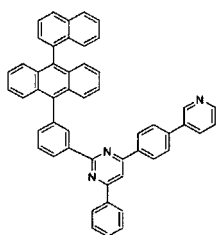
[Chemical Formula 311]
