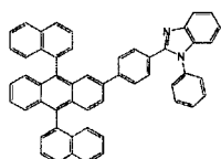
[Chemical Formula 280]
