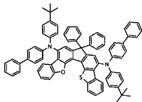
[Chemical Formula 245]
