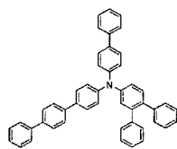
[Chemical Formula 87]
