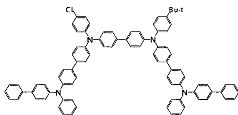
[Chemical Formula 364]
