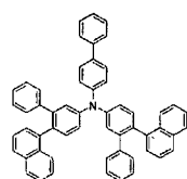
[Chemical Formula 120]
