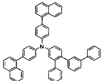
[Chemical Formula 174]
