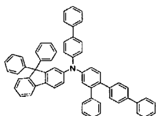
[Chemical Formula 390]
