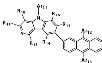
[Chemical Formula 11]
