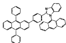
[Chemical Formula 275]
