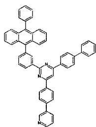
[Chemical Formula 306]
