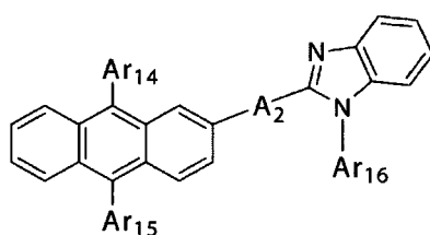
[Chemical Formula 7]
