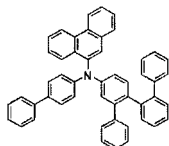
[Chemical Formula 401]
