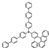
[Chemical Formula 103]
