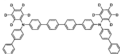
[Chemical Formula 350]
