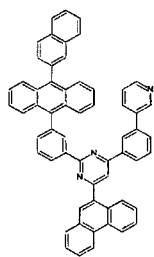
[Chemical Formula 298]
