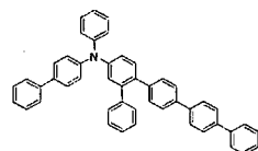
[Chemical Formula 57]
