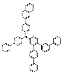
[Chemical Formula 170]
