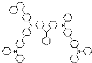
[Chemical Formula 368]
