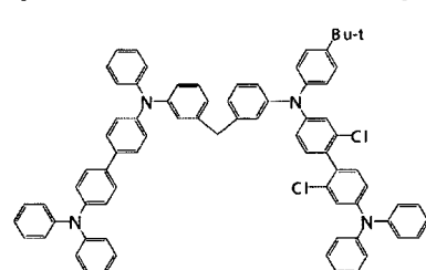
[Chemical Formula 367]
