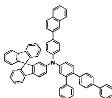
[Chemical Formula 209]
