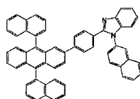
[Chemical Formula 281]
