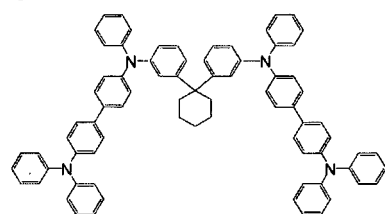
[Chemical Formula 365]
