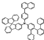
[Chemical Formula 207]
