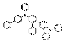
[Chemical Formula 59]
