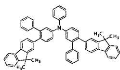
[Chemical Formula 132]
