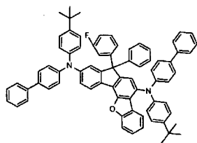
[Chemical Formula 242]
