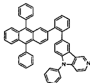
[Chemical Formula 263]
