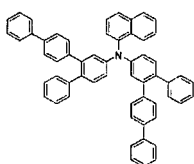
[Chemical Formula 149]
