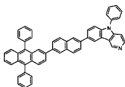
[Chemical Formula 267]
