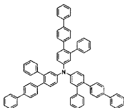
[Chemical Formula 156]
