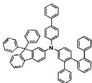
[Chemical Formula 193]
