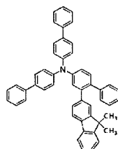
[Chemical Formula 112]
