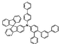
[Chemical Formula 199]
