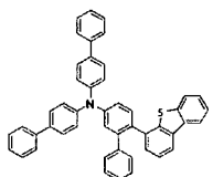
[Chemical Formula 38]
