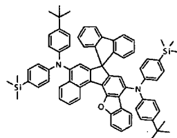
[Chemical Formula 233]
