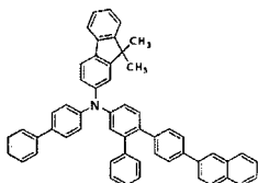
[Chemical Formula 189]
