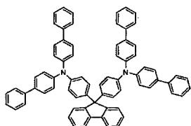
[Chemical Formula 325]
