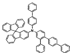
[Chemical Formula 198]
