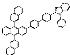
[Chemical Formula 270]
