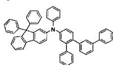
[Chemical Formula 195]
