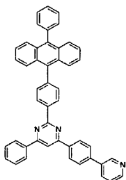
[Chemical Formula 309]
