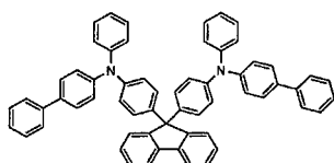
[Chemical Formula 321]
