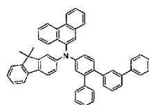
[Chemical Formula 225]
