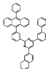
[Chemical Formula 290]
