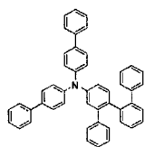
[Chemical Formula 31]
