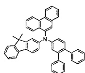
[Chemical Formula 223]
