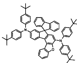
[Chemical Formula 420]
