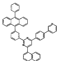
[Chemical Formula 301]
