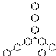
[Chemical Formula 99]
