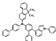
[Chemical Formula 83]
