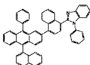
[Chemical Formula 271]
