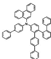
[Chemical Formula 222]
