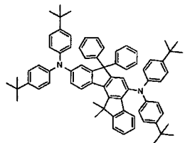
[Chemical Formula 246]
