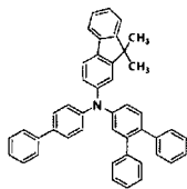
[Chemical Formula 75]
