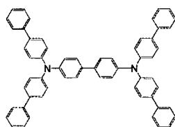
[Chemical Formula 314]
