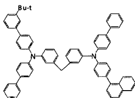
[Chemical Formula 323]
