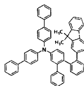
[Chemical Formula 47]
