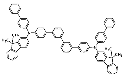
[Chemical Formula 354]
