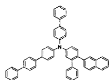
[Chemical Formula 89]
