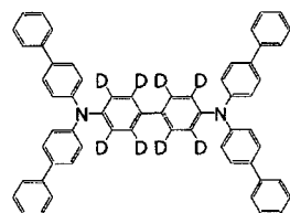
[Chemical Formula 334]
