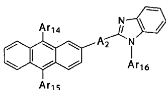
[Chemical Formula 7]
