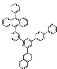
[Chemical Formula 302]
