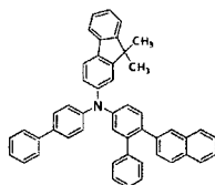
[Chemical Formula 77]
