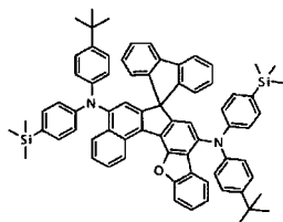
[Chemical Formula 408]
