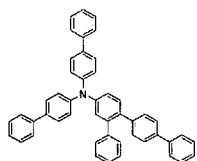
[Chemical Formula 29]
