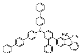
[Chemical Formula 90]
