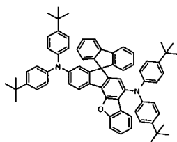
[Chemical Formula 402]
