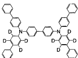
[Chemical Formula 331]
