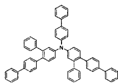
[Chemical Formula 123]
