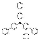
[Chemical Formula 27]
