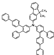
[Chemical Formula 153]
