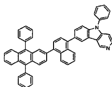
[Chemical Formula 266]
