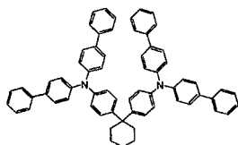
[Chemical Formula 320]
