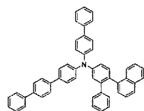
[Chemical Formula 88]
