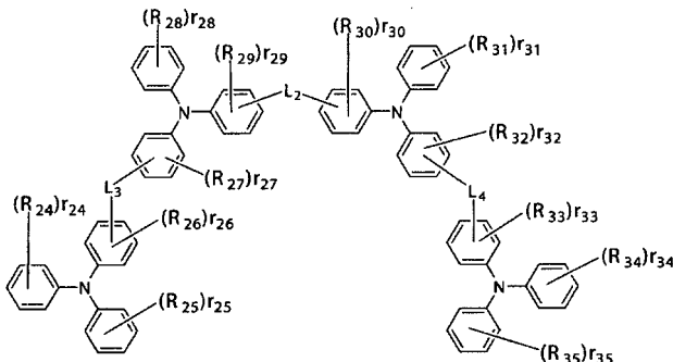
[Chemical Formula 19]
