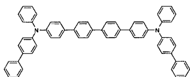
[Chemical Formula 346]
