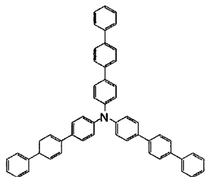
[Chemical Formula 429]
