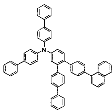
[Chemical Formula 162]
