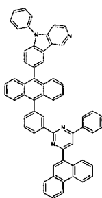
[Chemical Formula 305]
