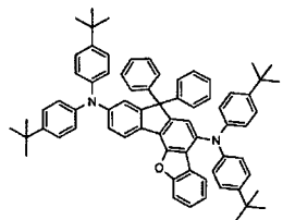
[Chemical Formula 238]
