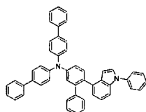
[Chemical Formula 36]
