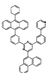
[Chemical Formula 295]
