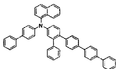
[Chemical Formula 70]
