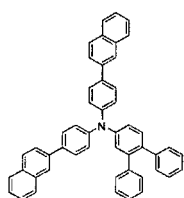
[Chemical Formula 179]
