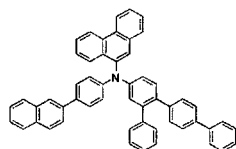
[Chemical Formula 219]
