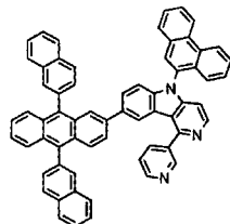
[Chemical Formula 258]
