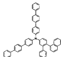
[Chemical Formula 100]
