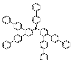
[Chemical Formula 147]
