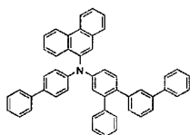
[Chemical Formula 400]
