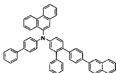
[Chemical Formula 217]
