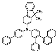
[Chemical Formula 76]
