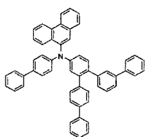
[Chemical Formula 221]
