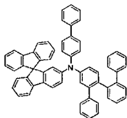
[Chemical Formula 200]
