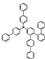
[Chemical Formula 161]
