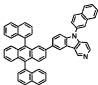
[Chemical Formula 257]
