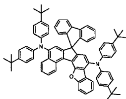
[Chemical Formula 404]
