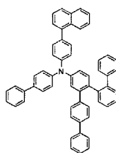
[Chemical Formula 167]
