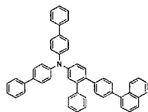
[Chemical Formula 39]
