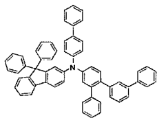
[Chemical Formula 192]
