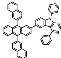
[Chemical Formula 252]
