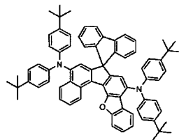
[Chemical Formula 229]
