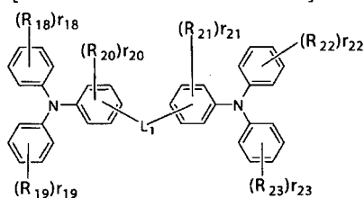
[Chemical Formula 12]
