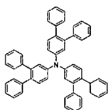
[Chemical Formula 154]
