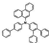
[Chemical Formula 212]
