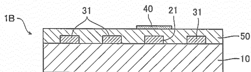
C-C' Cross Section
