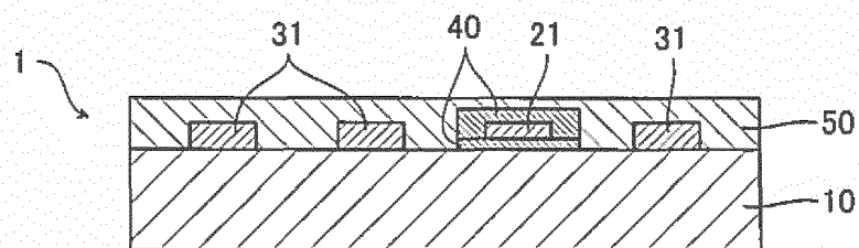
A-A' Cross Section
