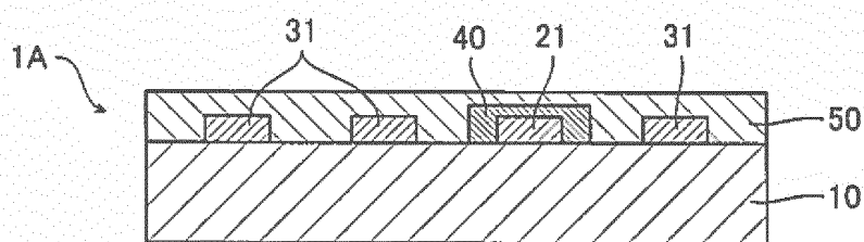
B-B' Cross Section
