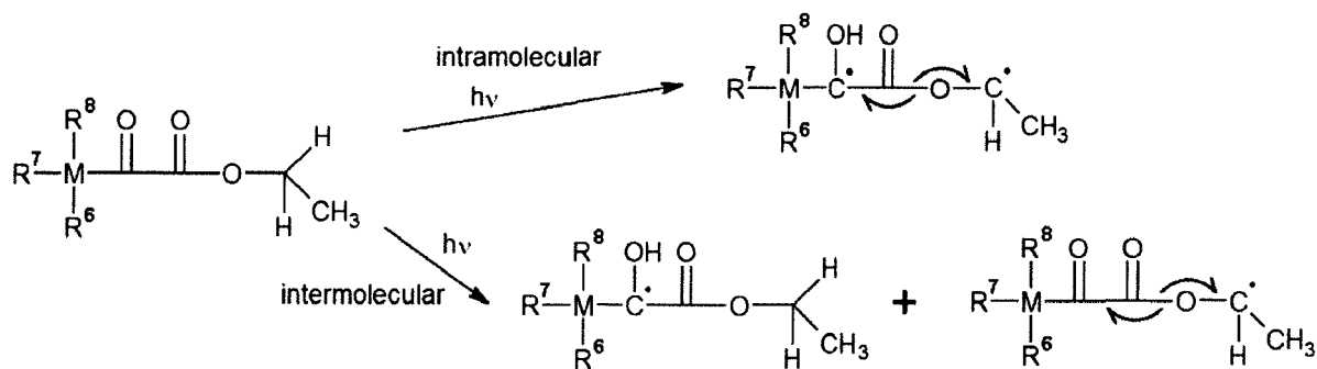
Scheme 5: hydrogen abstraction (intra- or intermolecular)
