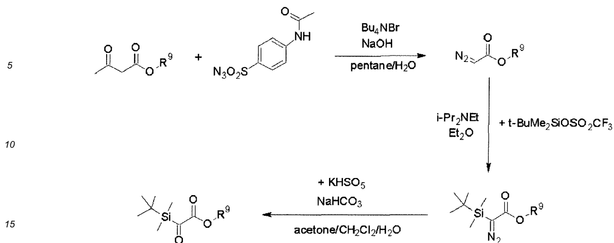
Scheme 2: Preparation of silylglyoxylates
