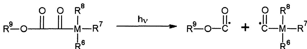
Scheme 4: cleavage of -O-C(=O)-C(=O)- moiety of a glyoxylate
