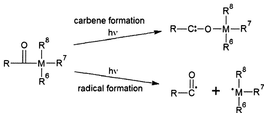
Scheme 3: carbene formation versus radical formation
