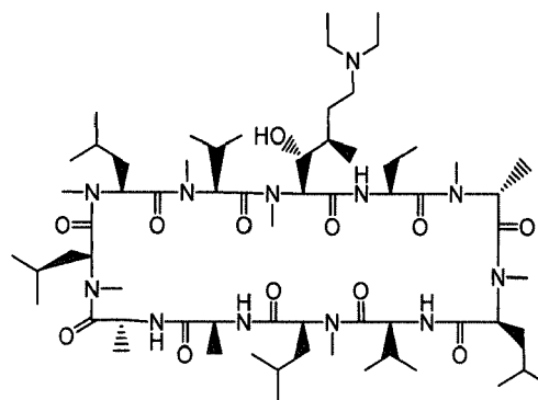
Compound M
