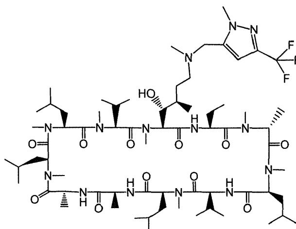
Compound DO
