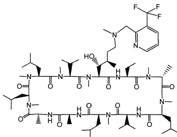
Compound DR
