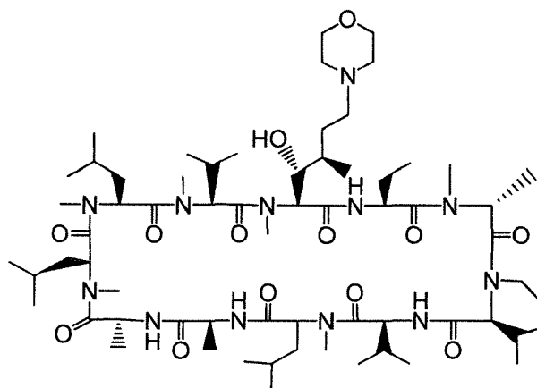
Compound EJ
