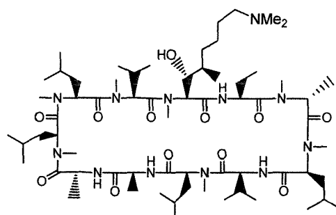
Compound KF
