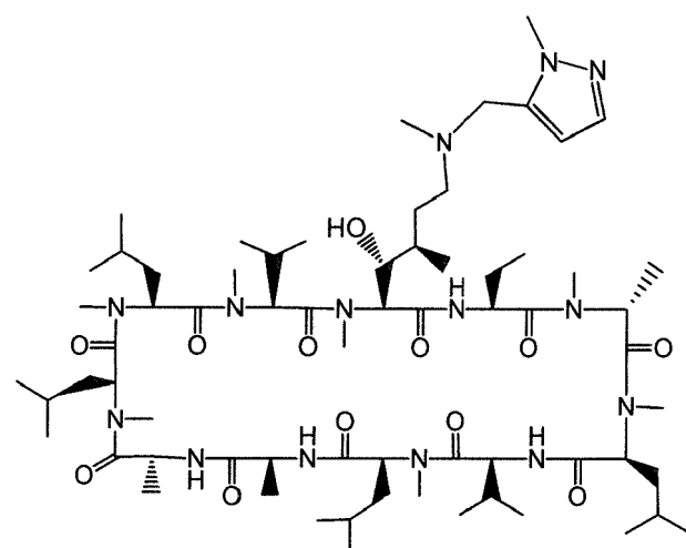
Compound DJ
