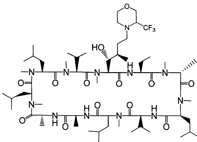
Compound EC
