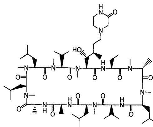
Compound N
