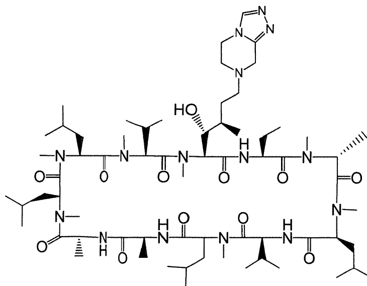
Compound DU
