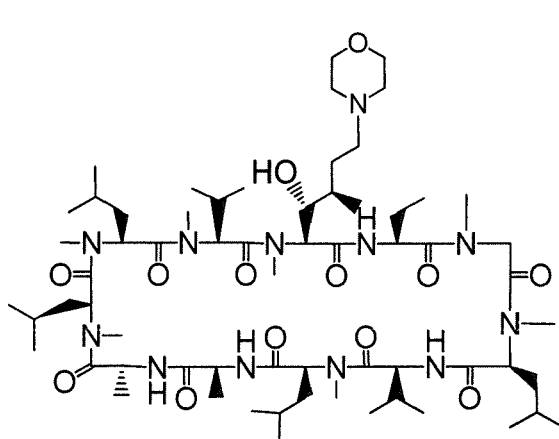
Compound A
