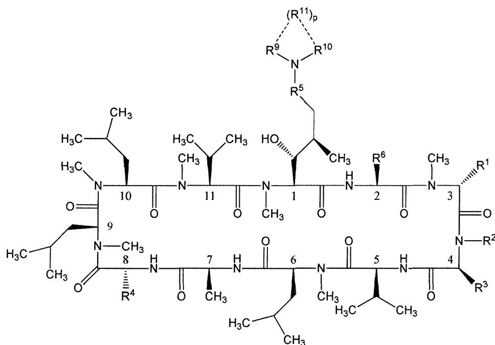
Formula I
