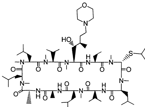
Compound I
