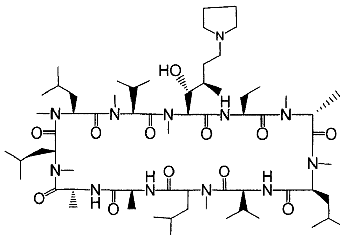
Compound EF
