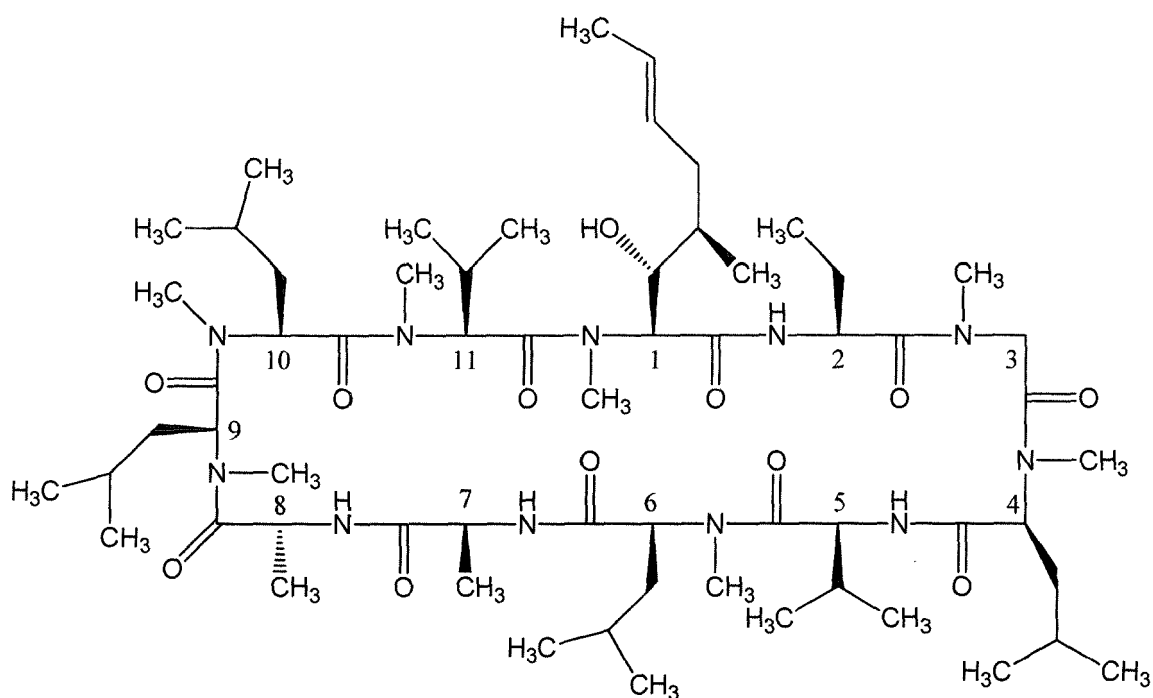
Cyclosporin A
