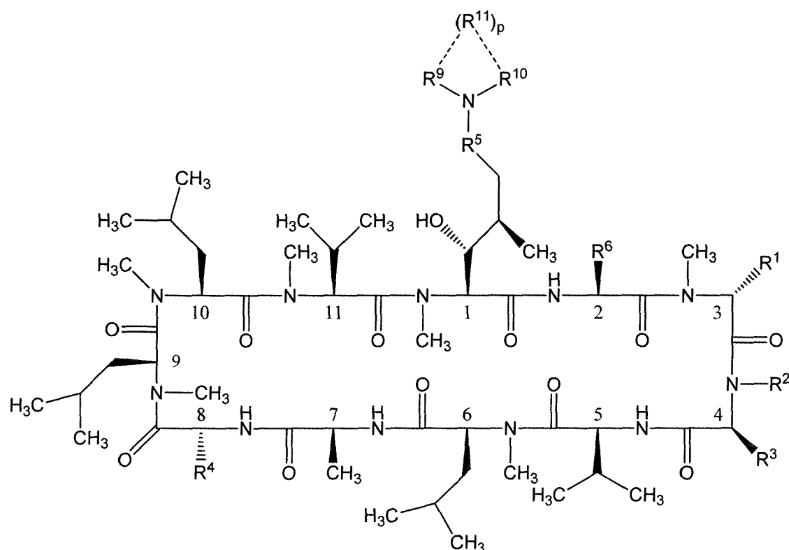
Formula I
