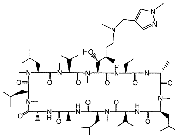
Compound DM
