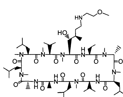
Compound AF
