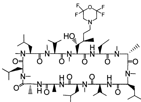
Compound EK
