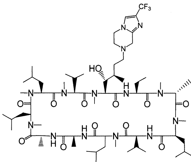
Compound EE
