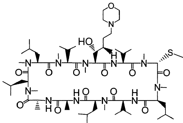
Compound AM
