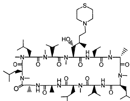
Compound J
