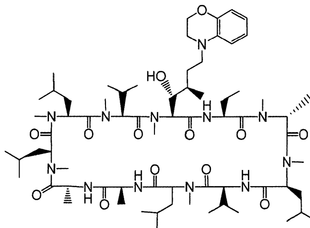
Compound DX
