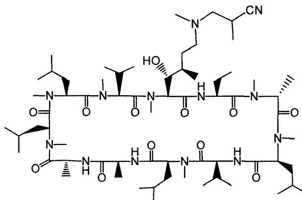
Compound DK
