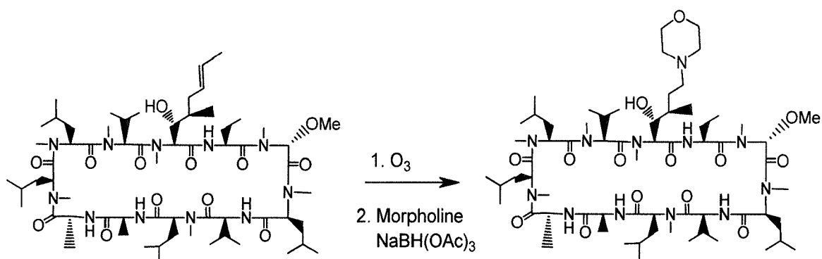
Compound B
