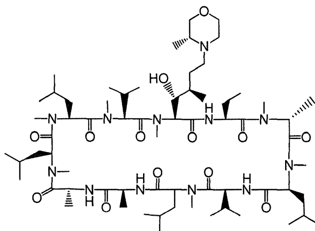
Compound DT
