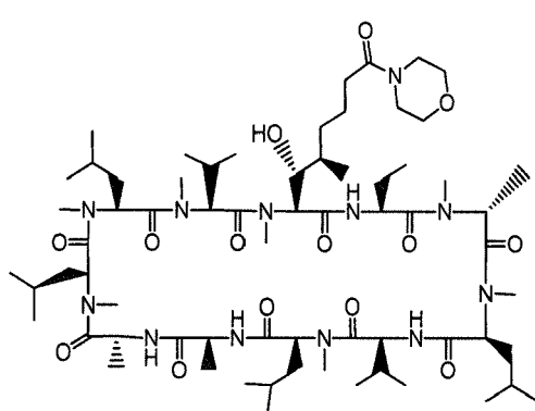
Compound H
