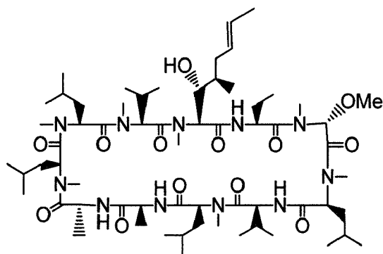
Intermediate 18
