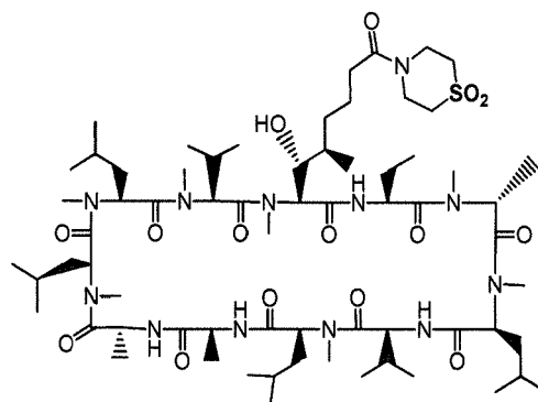
Compound Z
