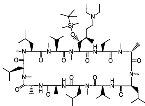
Intermediate 51
