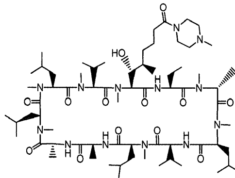
Compound T
