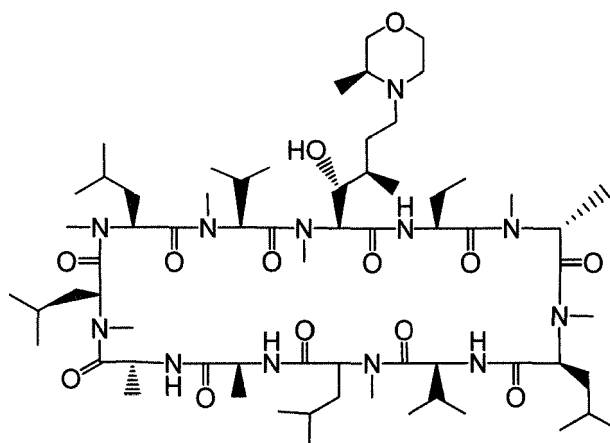
Compound DW
