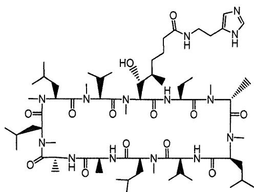
Compound Y
