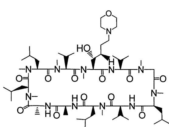
Compound AN
