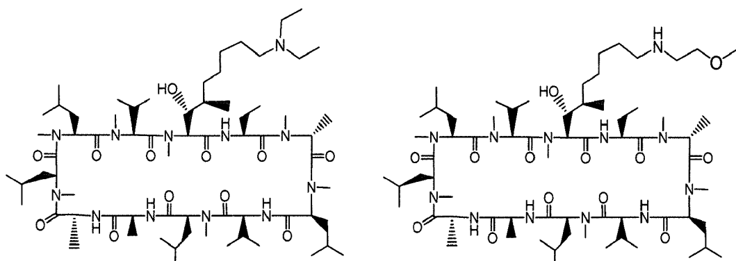
Compound AH
