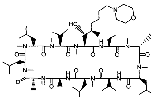
Compound KG
