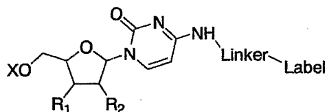
Cytidine N4-linker
