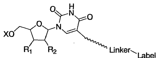
Uridine C5-linker
