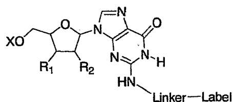
Guanosine N2-linker
