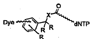
generic compound
