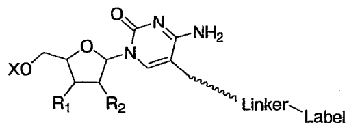
Cytidine C5-linker
