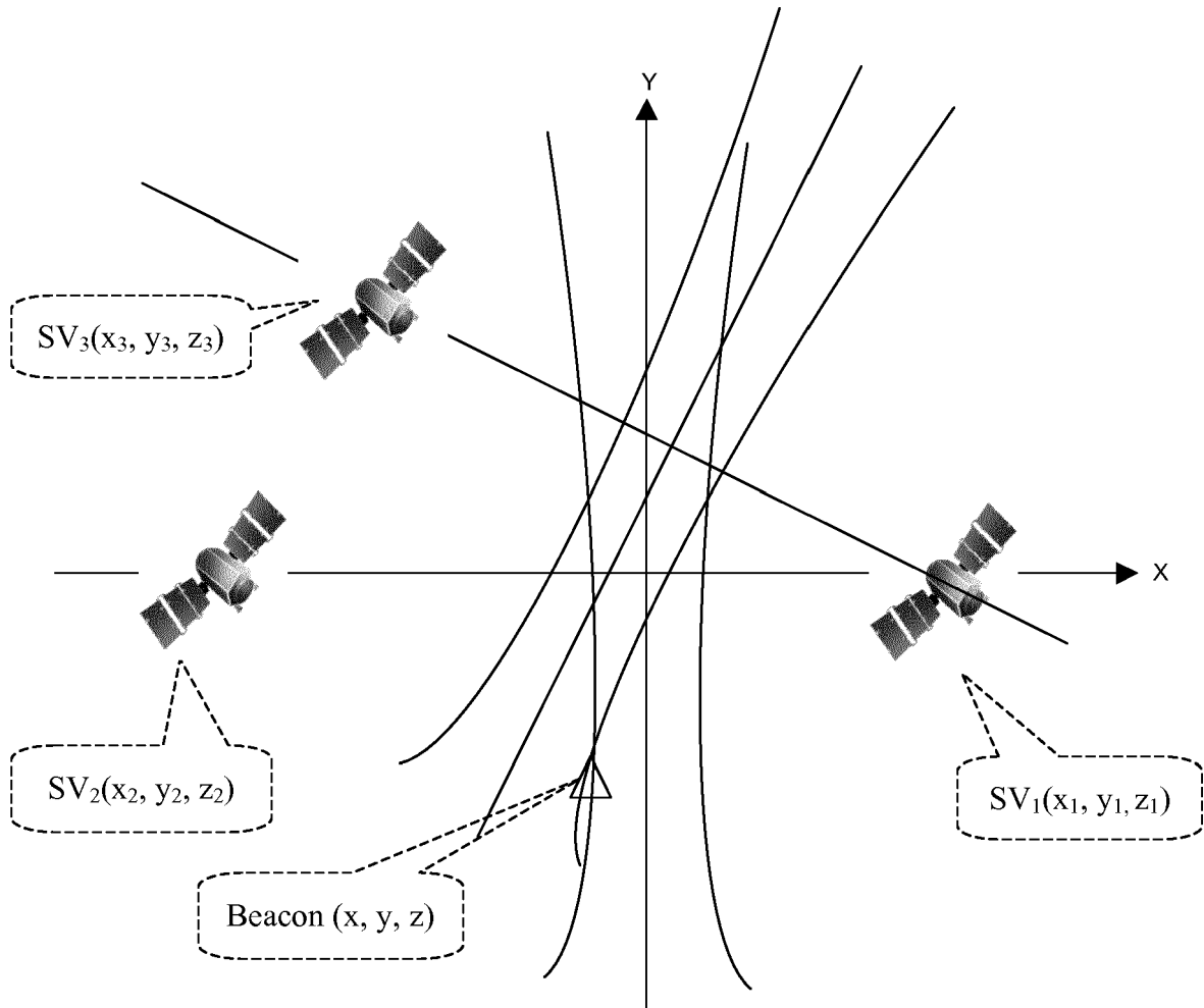
FIG.2 – Beacon Localization based on TDOA
