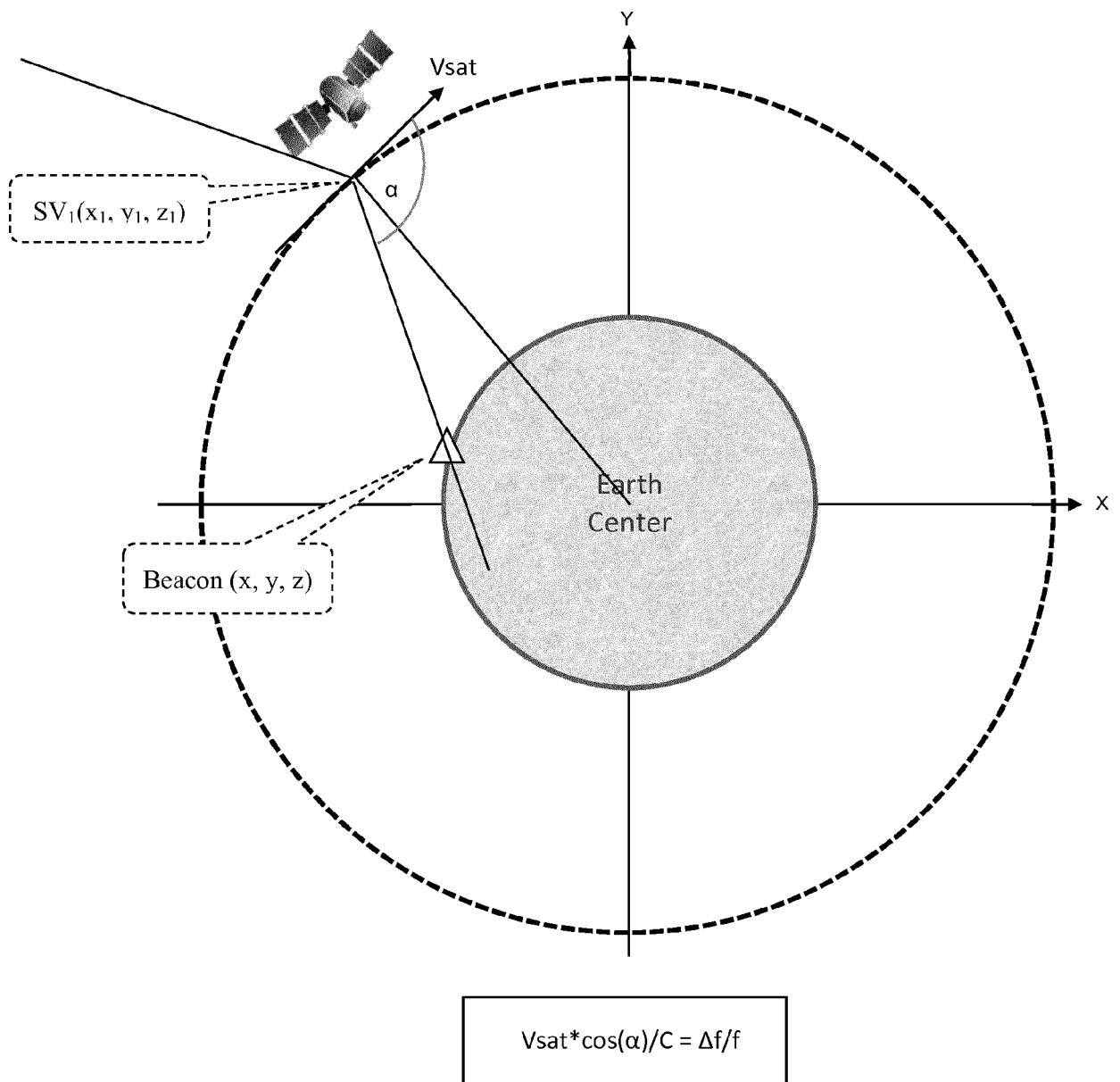
FIG.3 – Beacon Localization based on FOA
