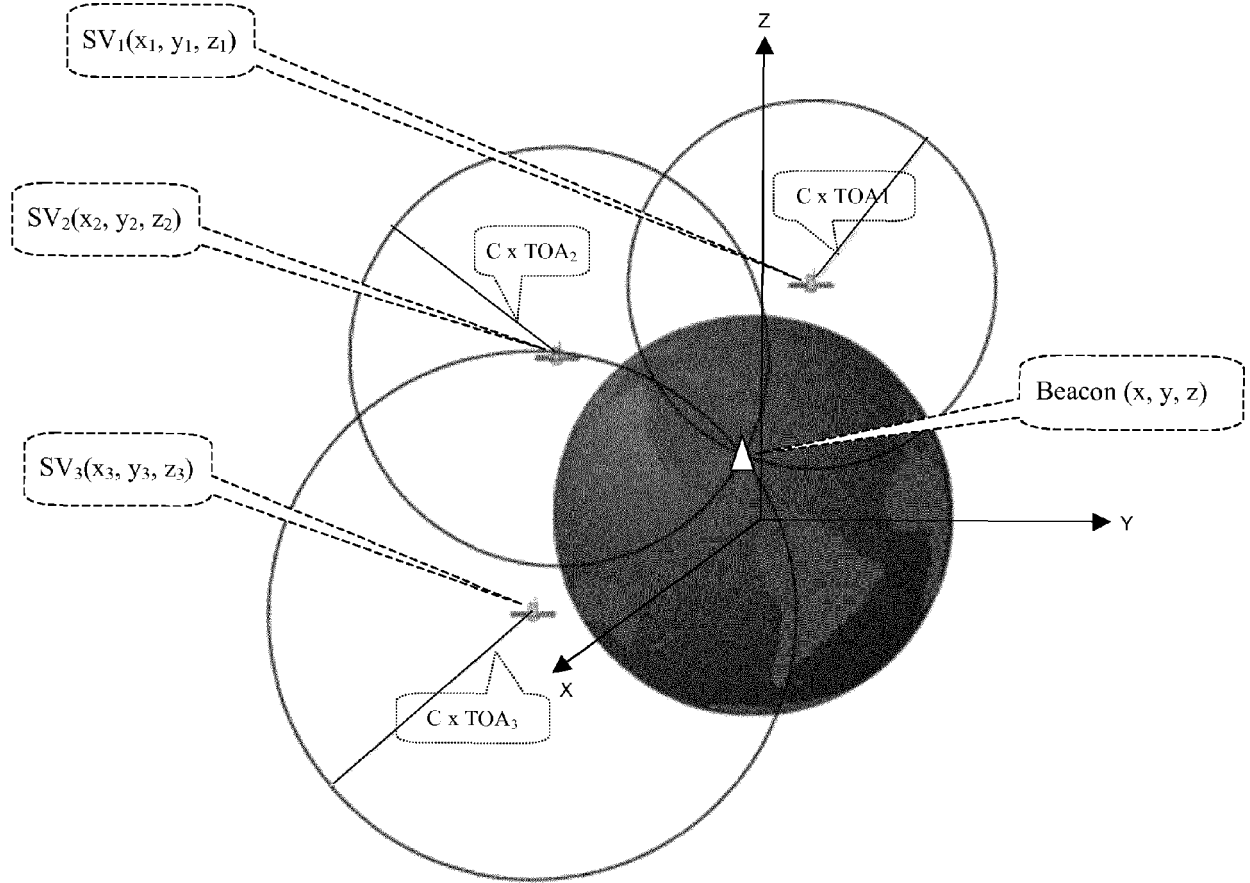
FIG.1 – Beacon Localization based on TOA
