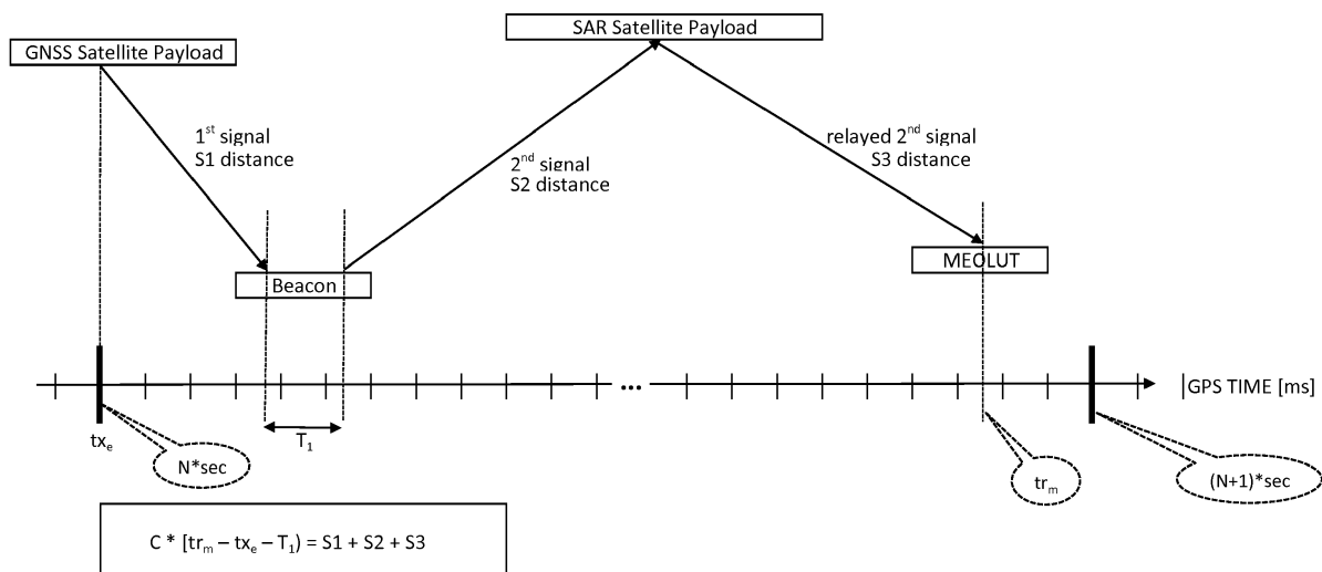
FIG.6 - TOA Measurement According to a 1 st Embodiment of the Present Invention
