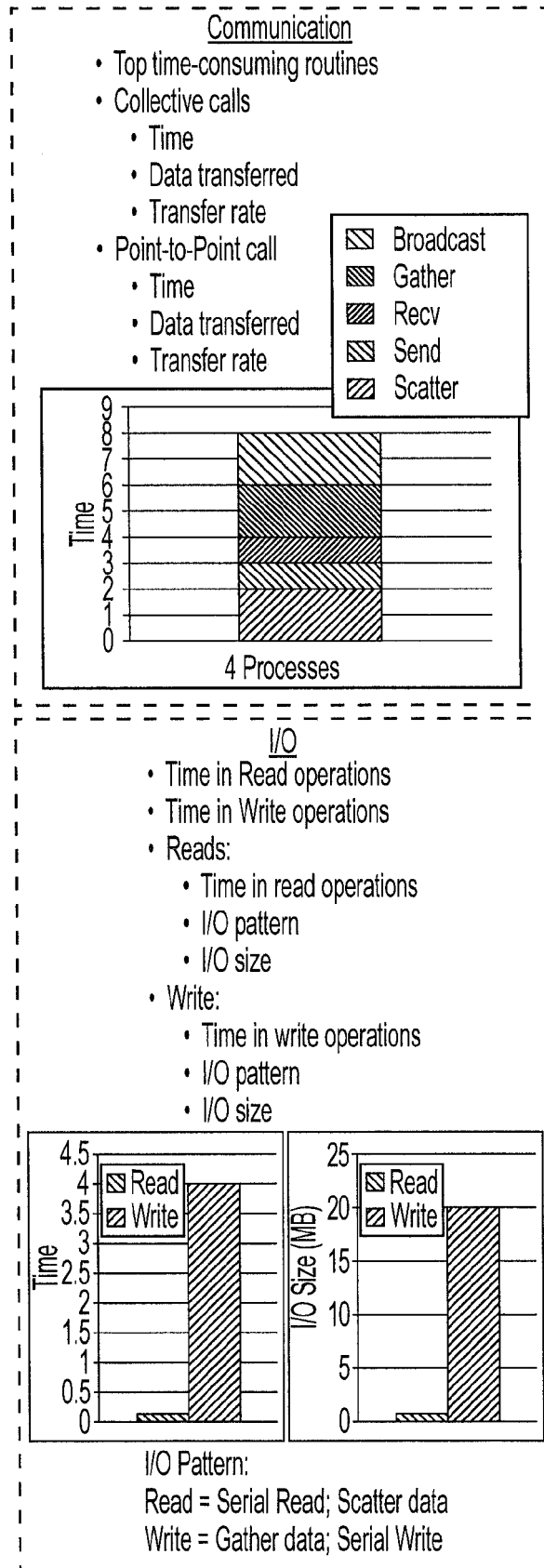
FIG. 10 (continued)
