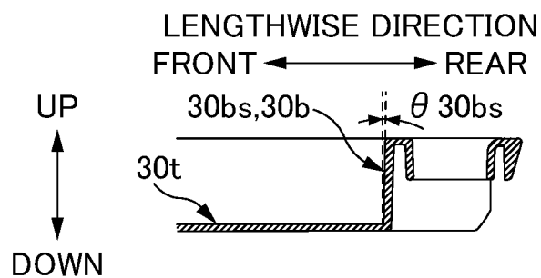
B-B SECTION
