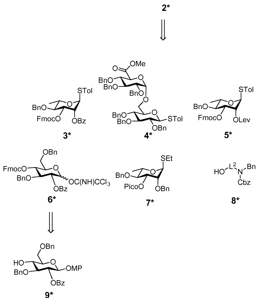
Scheme 4: Retrosynthetic analysis of a saccharide of general formula 2* .
