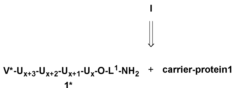
Scheme 1: Retrosynthetic analysis of the S. pneumoniae serotype 8 conjugates of general formula (I).
