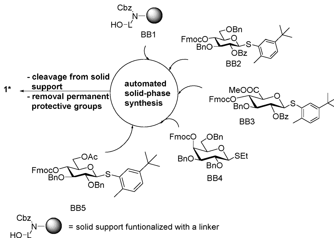
Scheme 2: Automated solid phase synthesis of saccharides of general formula 1*.
