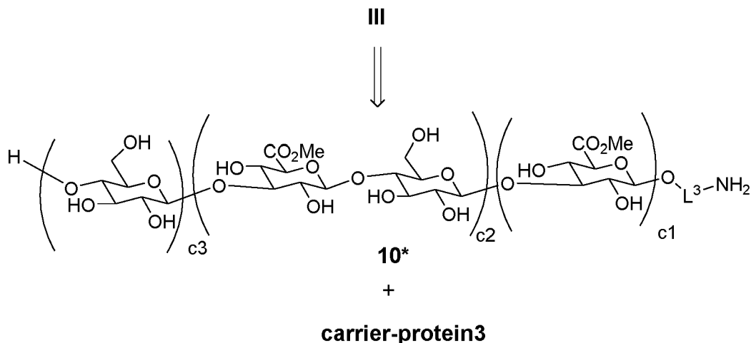
Scheme 1: Retrosynthetic analysis of the S. pneumoniae serotype 3 conjugates of general formula (III).
