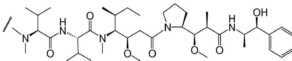
MMAE
