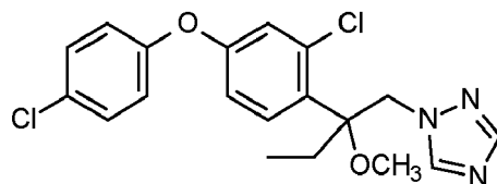
I-22 1-[2-[2-chloro-4-(4-chlorophenoxy)phenyl]-2-methoxy-pentyl]-1,2,4-triazole:
