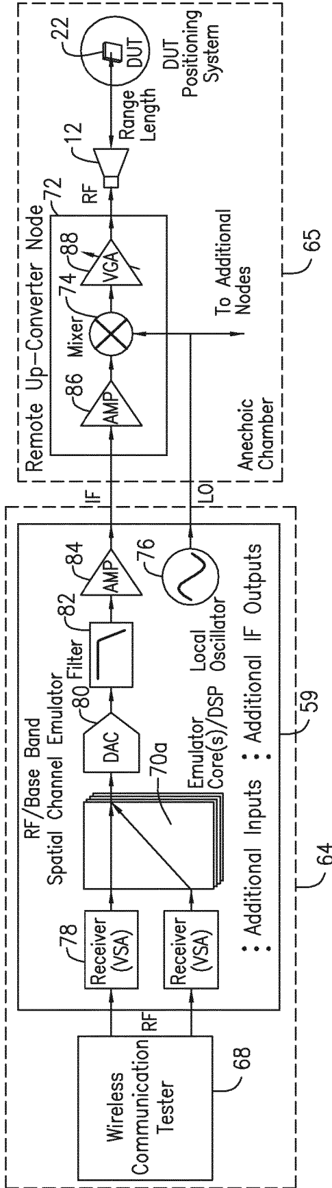
Individual Downlink Signal Chain Using Baseband IF to Remote RF Node
