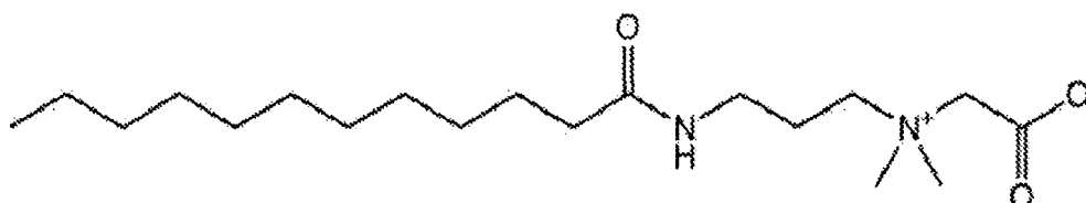
Structure of Cocoamidopropyl betaine
