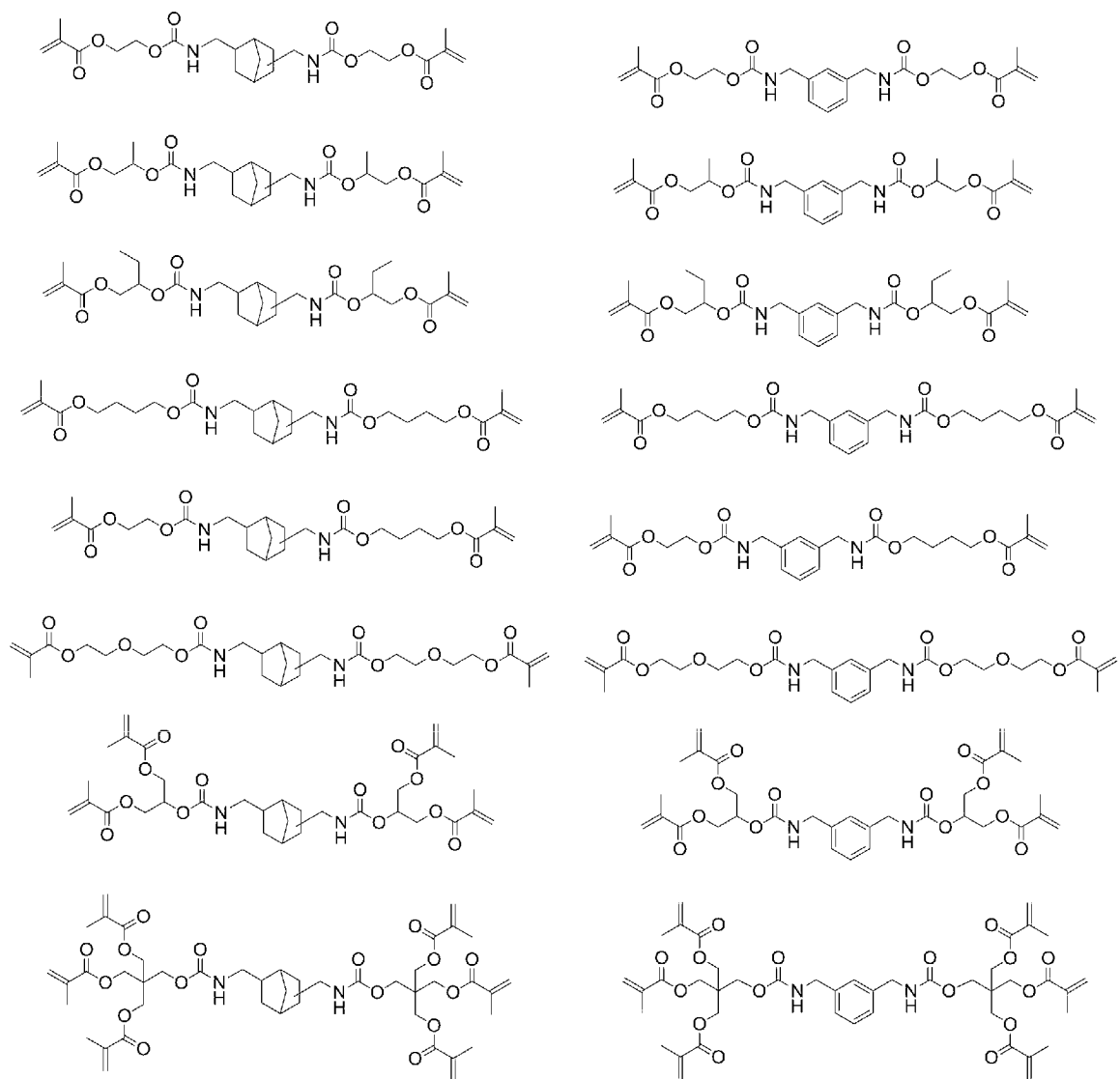
[Chem. 24]
