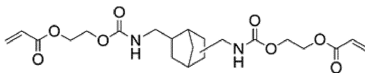
Compound 6d
