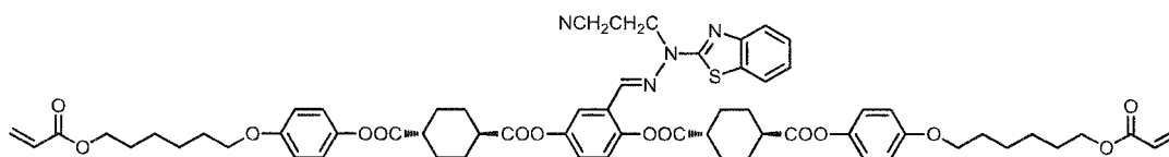
Polymerizable compound (IIIq)
