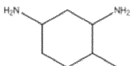
4-methylcyclohexane-1,4-diamine;
