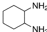
Cyclohexane-1,2-diamine;
