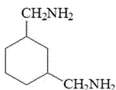
1, 3-bis(methylamine)-cyclohexane,;
