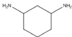
Cyclohexane-1,3-diamine;
