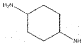
Cyclohexane-1,4-diamine;
