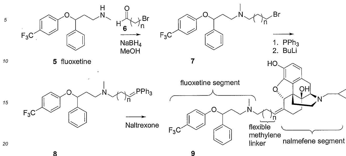
Scheme 1
