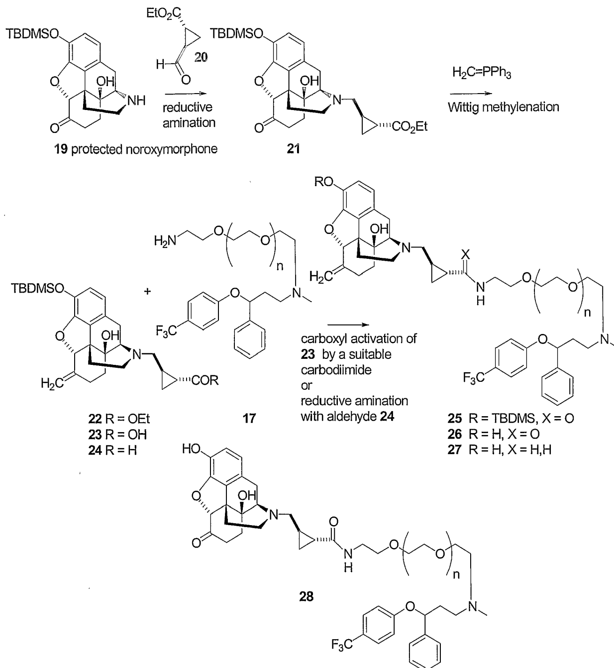
Scheme 4
