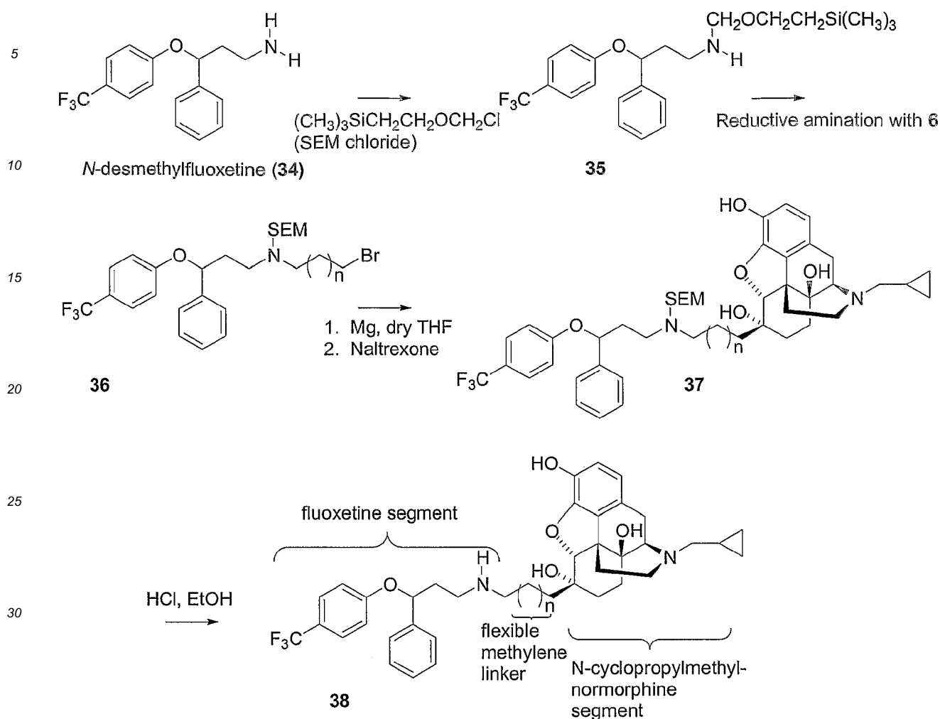
Scheme 7
