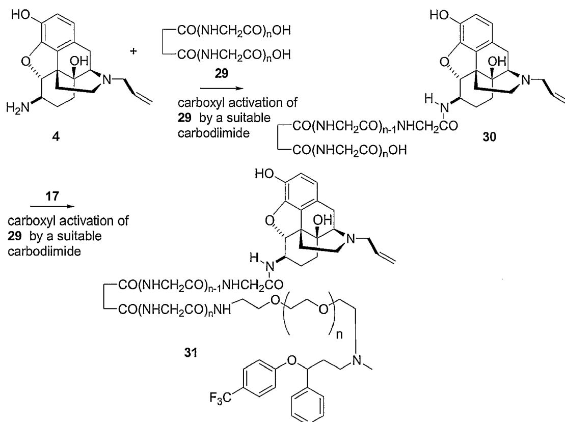
Scheme 5
