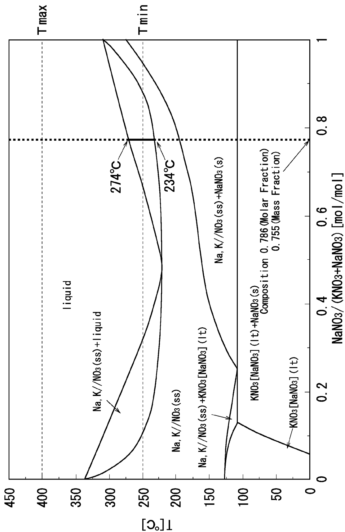
KNO 3 —NaNO 3 FIG.1b
