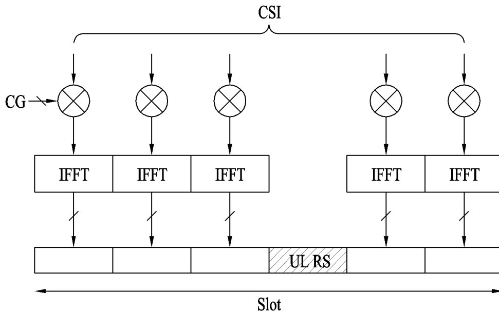
PUCCH format 2/2a/2b structure (extended CP)
