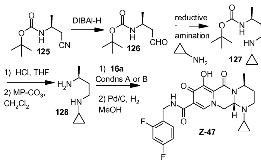
[Chemical formula 74]
