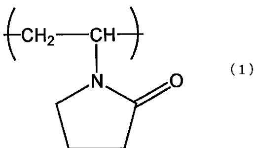
[Chem. 1]
