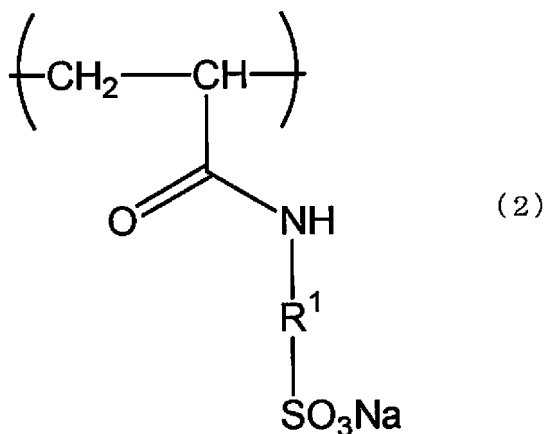
[Chem. 2]
