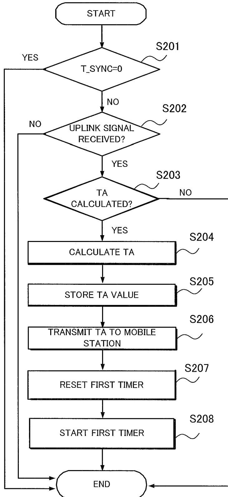
FIG. 16 DEEMED IN-SYNC STATE
