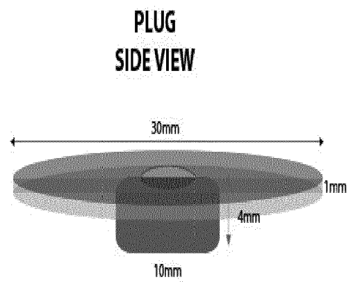
Fig. 3(a): Schematic Perspective Side View of an anchor plug
