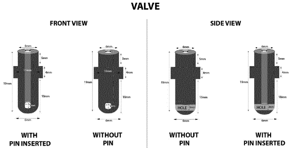
Fig. 4: Schematic Front and Side View of a Dual Function Valve with and without Inserted Pin
