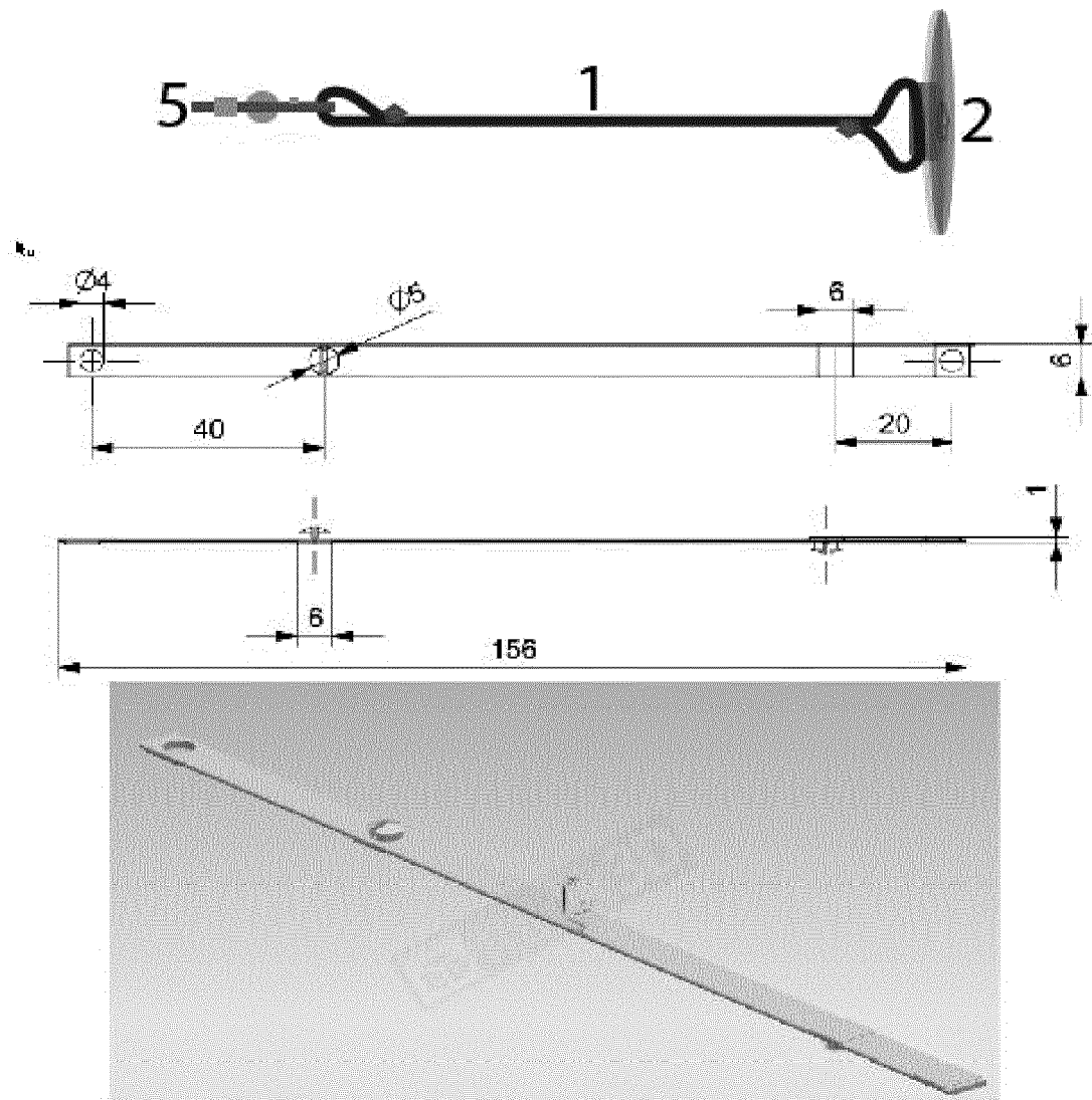
Fig. 2: Schematic Perspective View of cables that are locked to the anchor plugs on one side and electronic component on the other side
