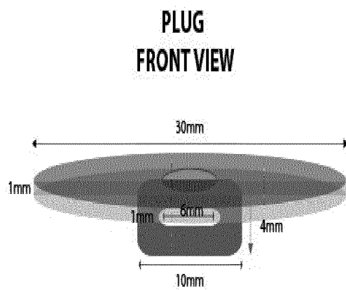
Fig. 3: Schematic Perspective Front View of an anchor plug
