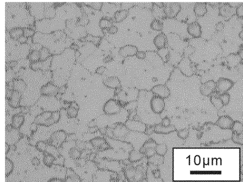
HOT WORKED MATERIAL A (DISK AFTER FORMING)
