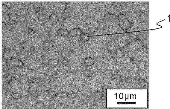
HOT WORKING MATERIAL A (MATERIAL BEFORE FORMING)
