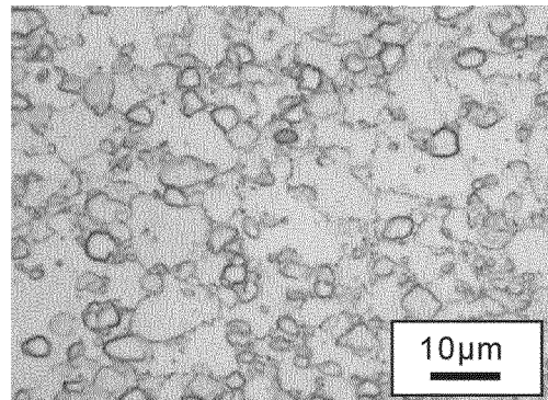
HOT WORKED MATERIAL B (DISK AFTER FORMING)
