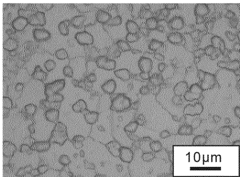
HOT WORKING MATERIAL B (MATERIAL BEFORE FORMING)
