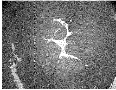
Dp4e4mT-HCl 1.5 mg
