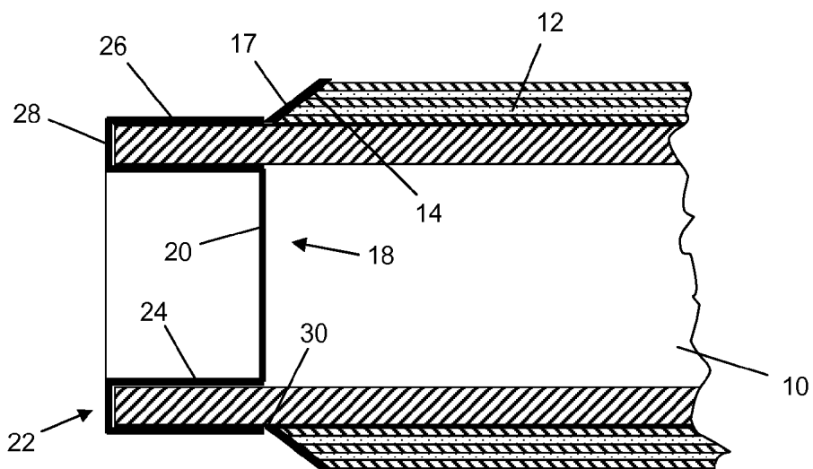
Figure 3 PRIOR ART
