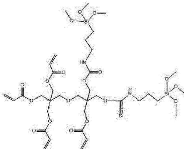
[Chemical Formula 14]
