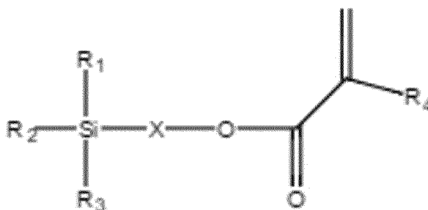
[Chemical Formula 15]
