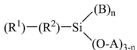
[Chemical Formula 14]
