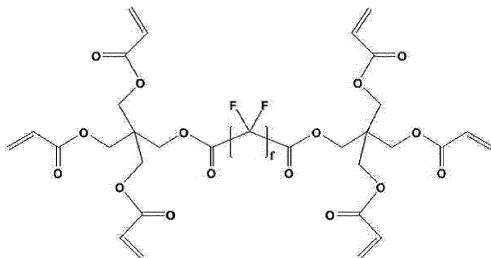
[Chemical Formula 5]
