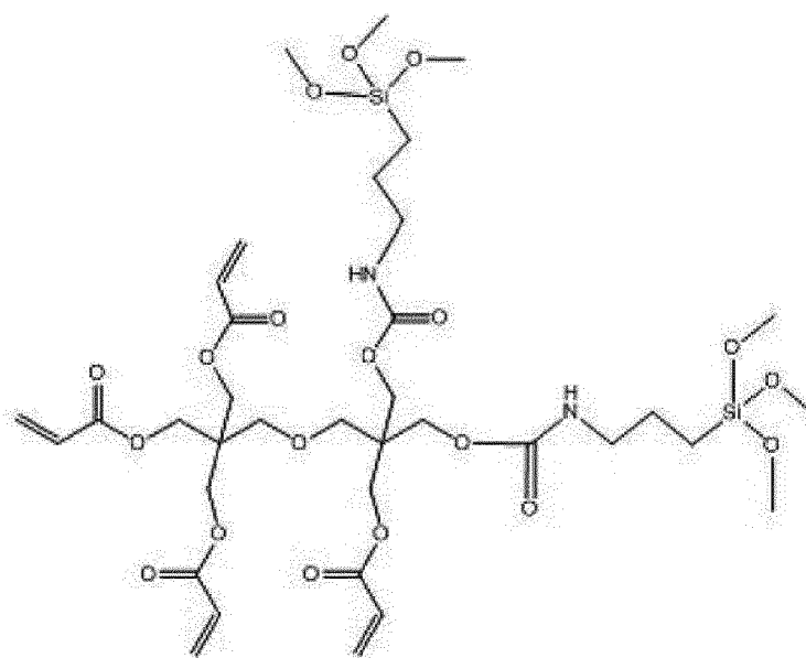
[Chemical Formula 14]
