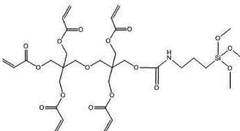
[Chemical Formula 12]
