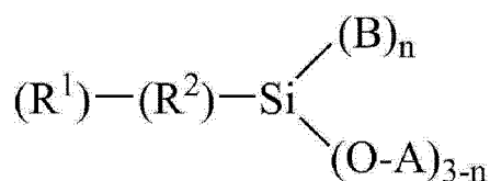
[Chemical Formula 14]
