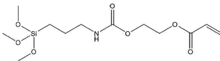
[Chemical Formula 11]
