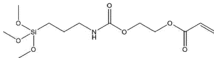
[Chemical Formula 12]
