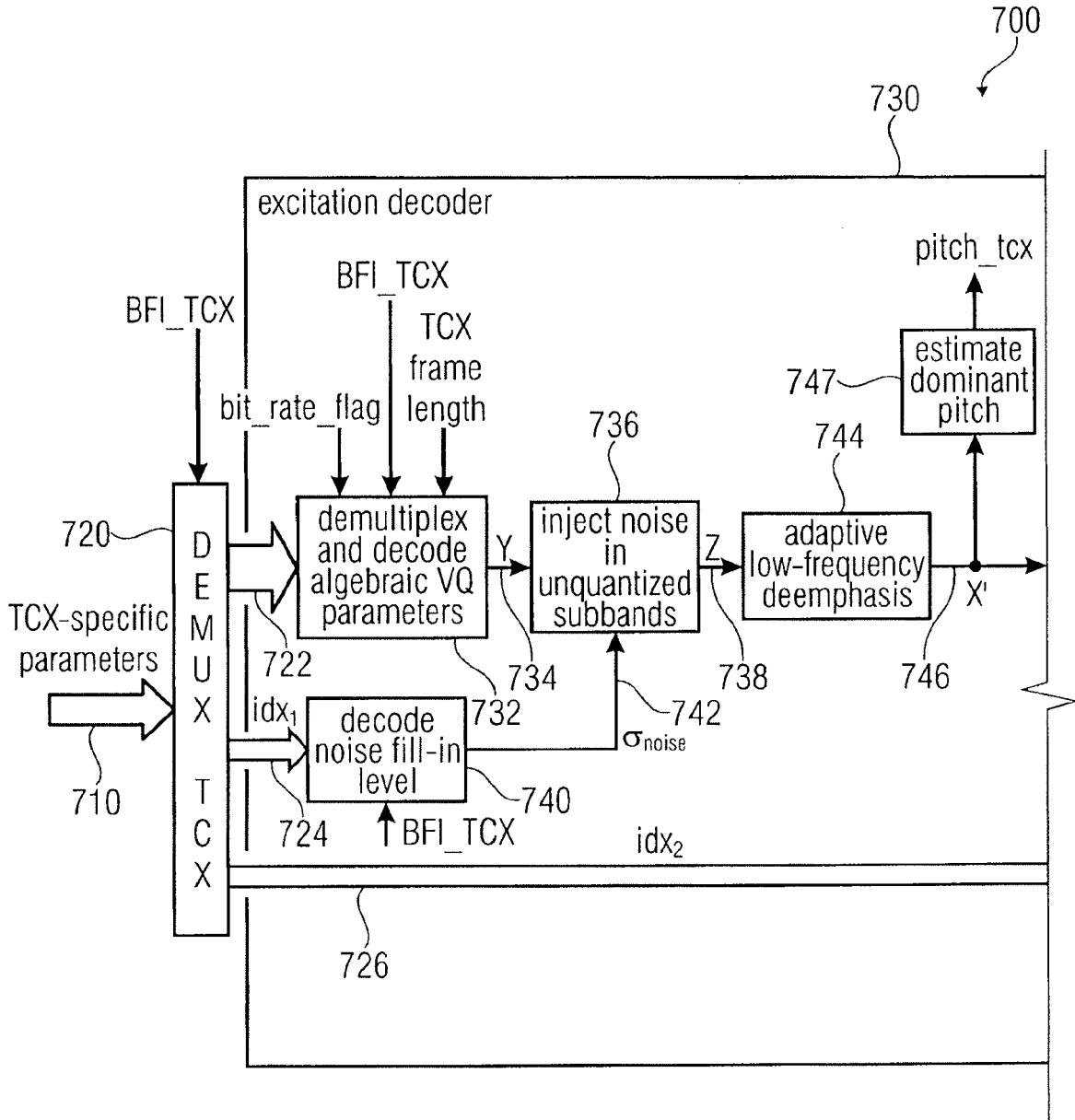
Block diagram of the TCX decoder
