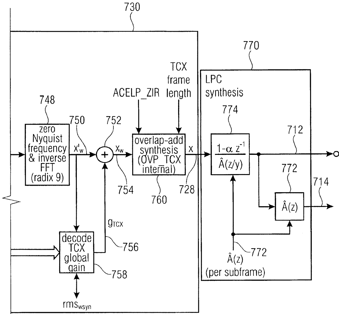
TCX decoding in normal or in partial packet loss.
