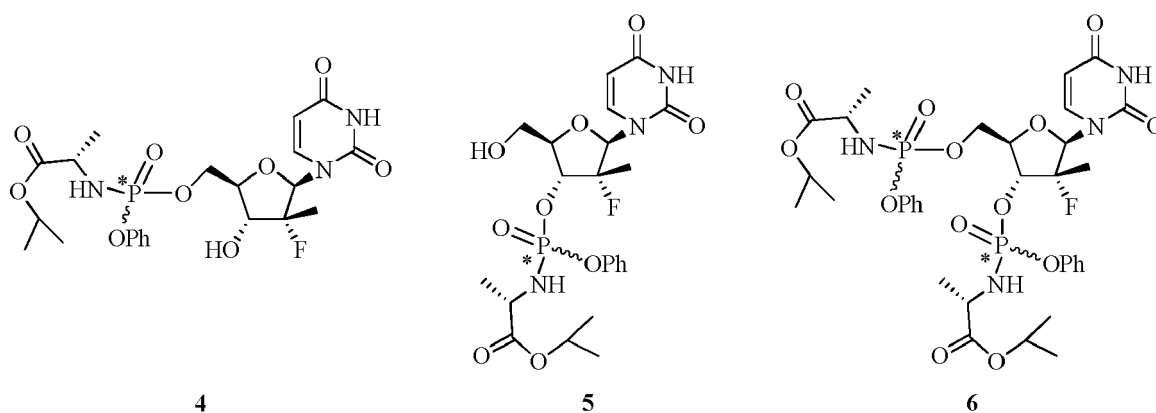
5'-O-phosphoramidate (2 diastereomers)
