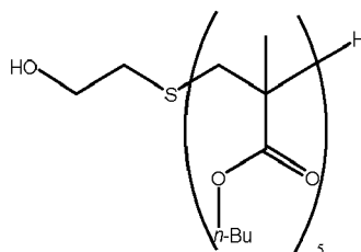
Hydroxylated BMA Oligomer, dp = 5
