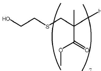
Hydroxylated MMA Oligomer, dp = 5
