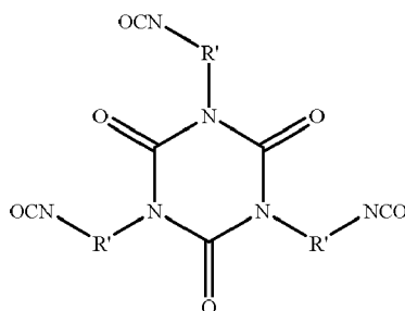
Isocyanurate trimer
