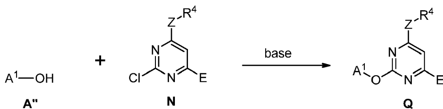
General Scheme 8
