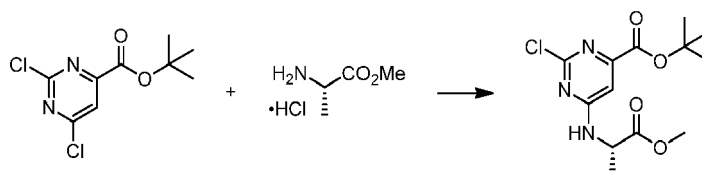
Scheme 11
