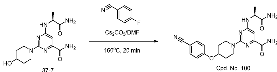
Scheme 84
