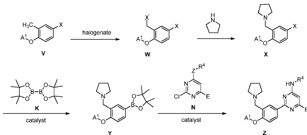
General Scheme 10
