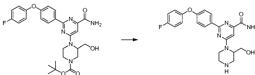
Scheme 24
