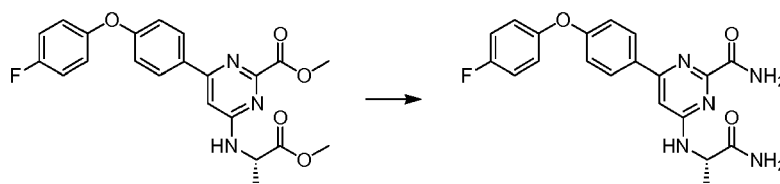
Scheme 41
