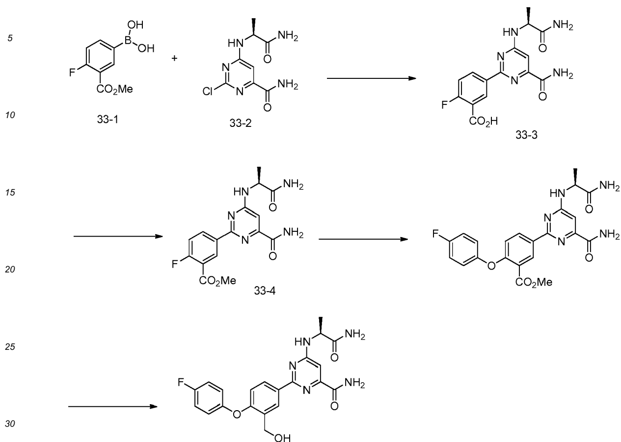
Scheme 76
