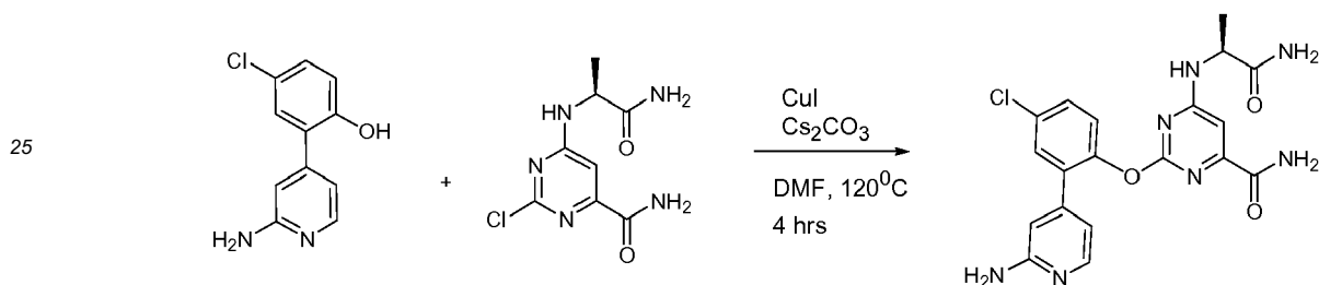
Scheme 48
