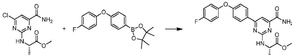
Scheme 37
