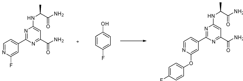
Scheme 50
