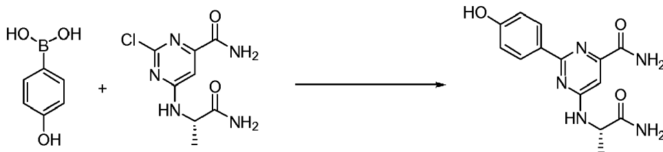
Scheme 45
