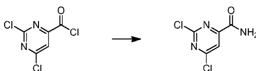
Scheme 3
