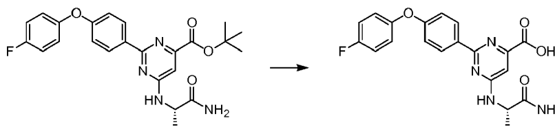
Scheme 16
