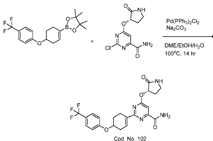
Scheme 82
