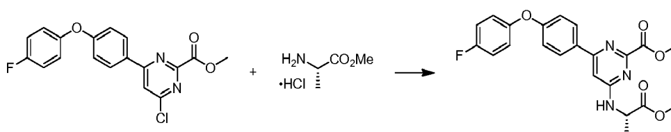
Scheme 40
