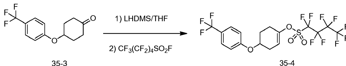
Scheme 79
