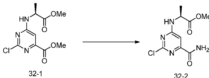
Scheme 73
