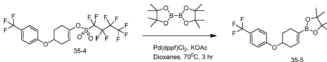
Scheme 80
