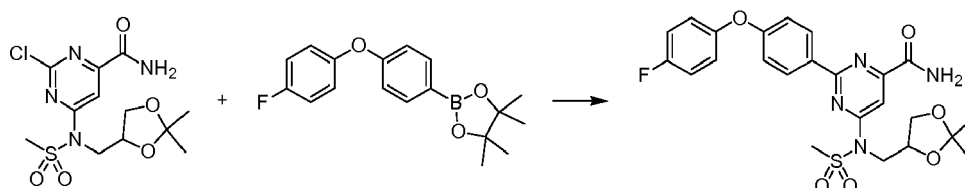
Scheme 35
