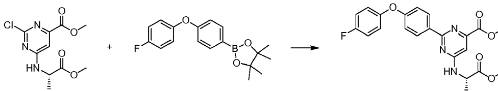
Scheme 20
