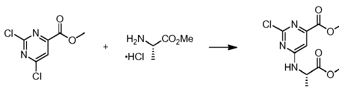
Scheme 17
