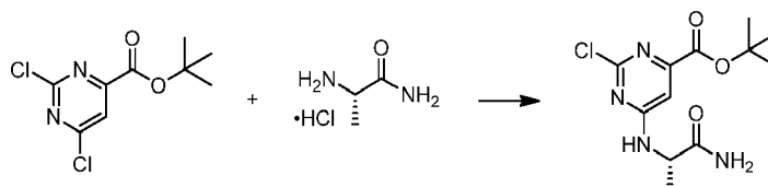
Scheme 14
