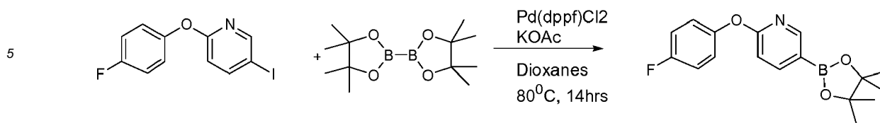
Scheme 52
