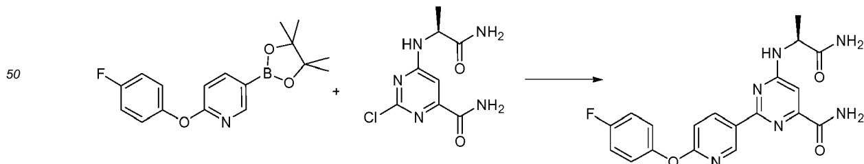
Scheme 53
