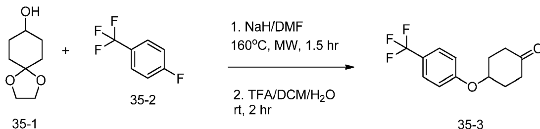
Scheme 78
