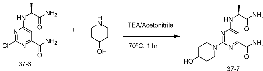
Scheme 83
