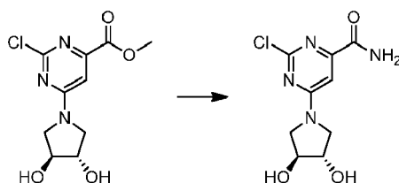
Scheme 59
