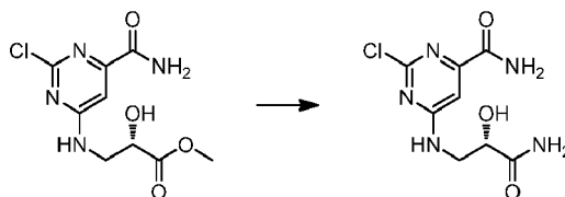
Scheme 29
