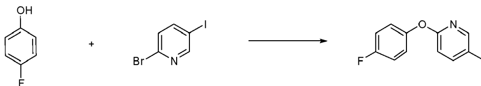
Scheme 51
