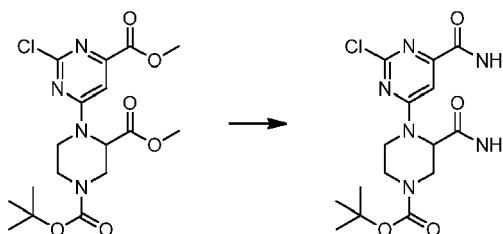
Scheme 62
