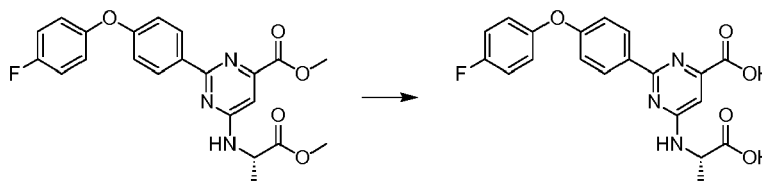
Scheme 21
