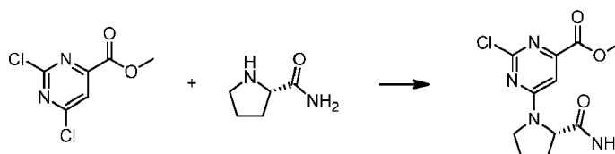
Scheme 55
