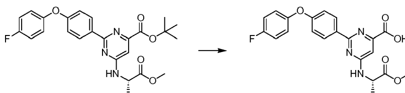
Scheme 13
