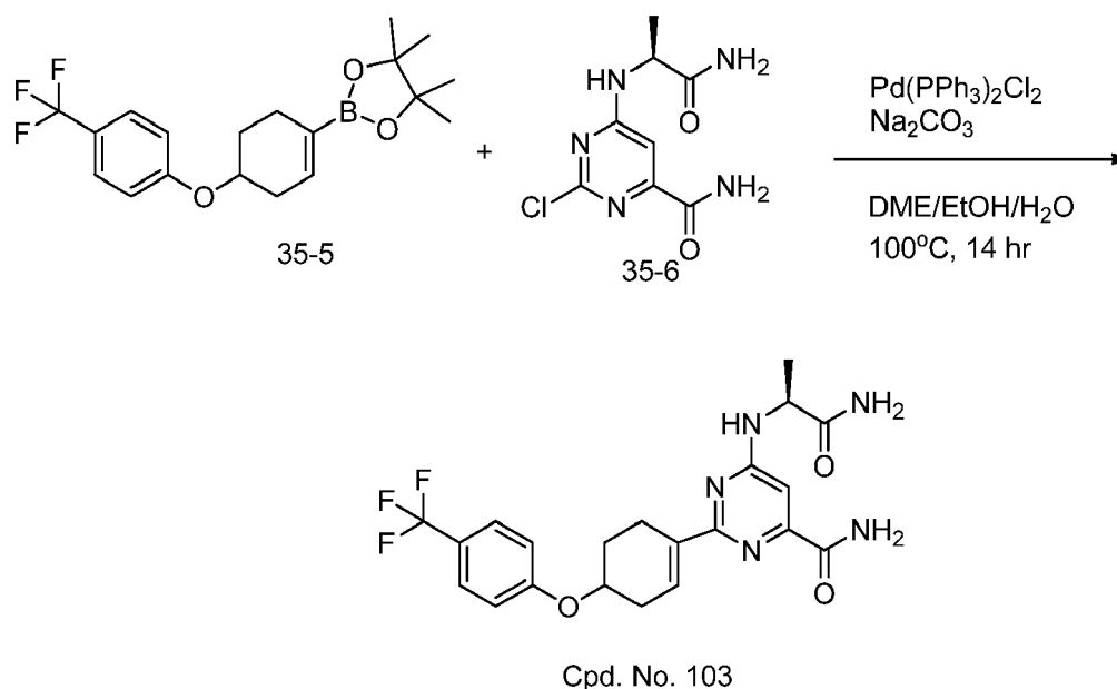
Scheme 81
