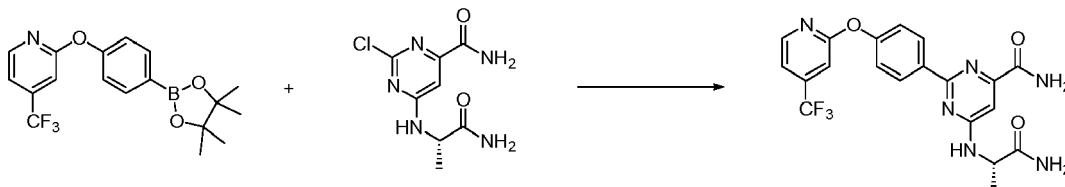
Scheme 44
