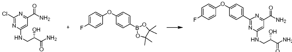
Scheme 30
