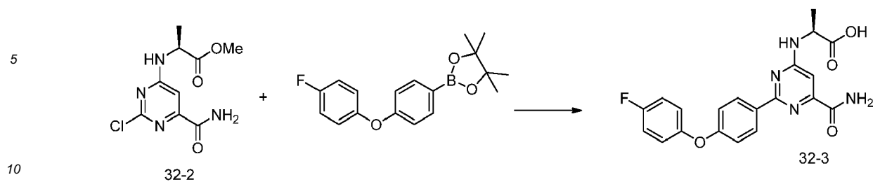
Scheme 74
