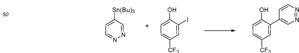
Scheme 49
