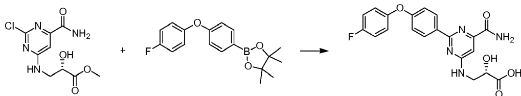
Scheme 31
