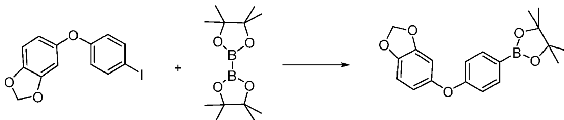
Scheme 71
