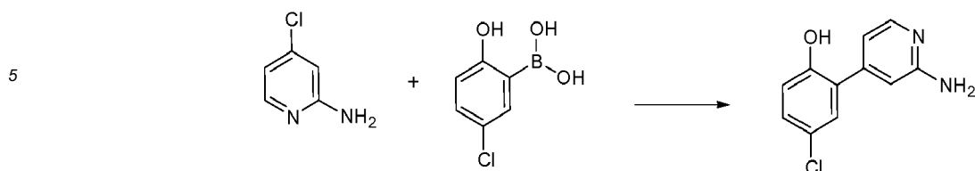
Scheme 47
