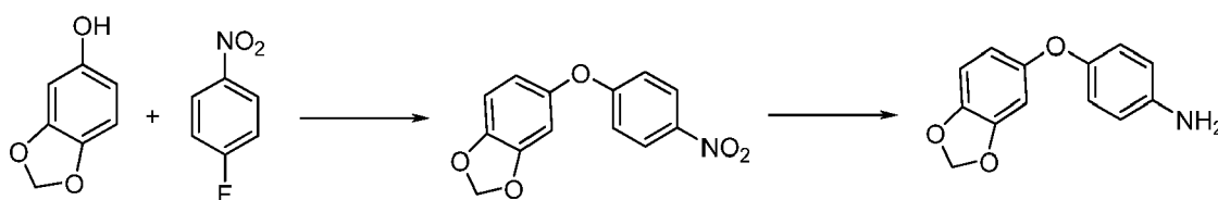
Scheme 69
