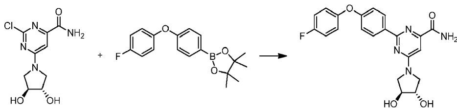
Scheme 60
