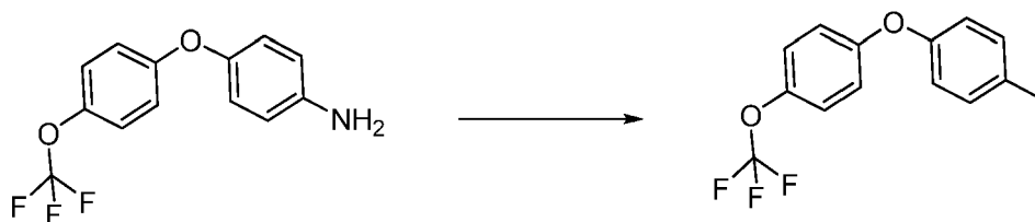
Scheme 66
