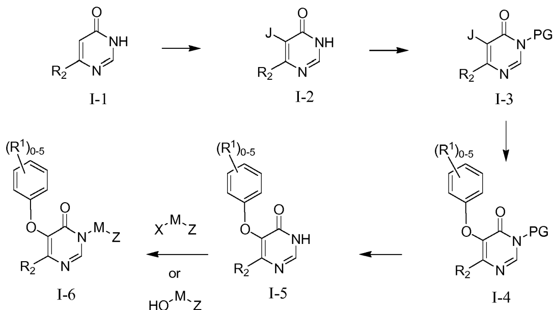
Scheme I
