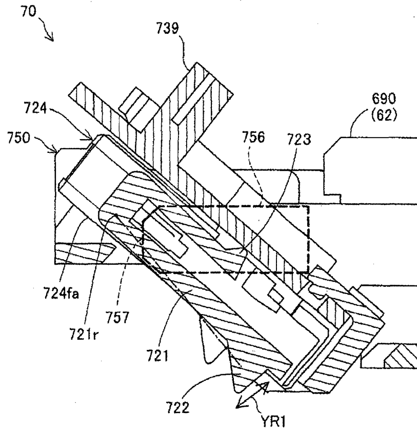
17-17 CROSS-SECTIONAL VIEW
