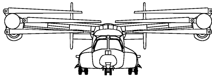
Fig.1C (PRIOR ART)
