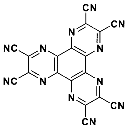
[HAT]
