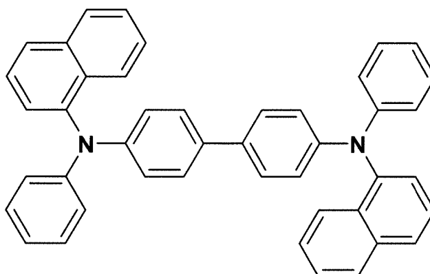
[NPB]
