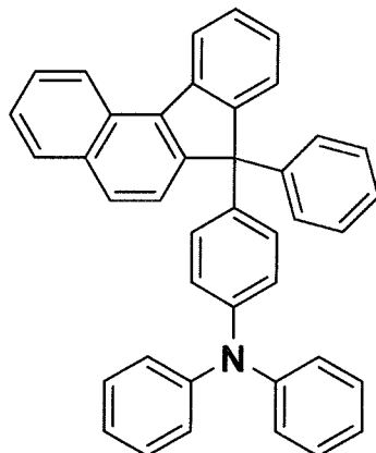
[ET6]
