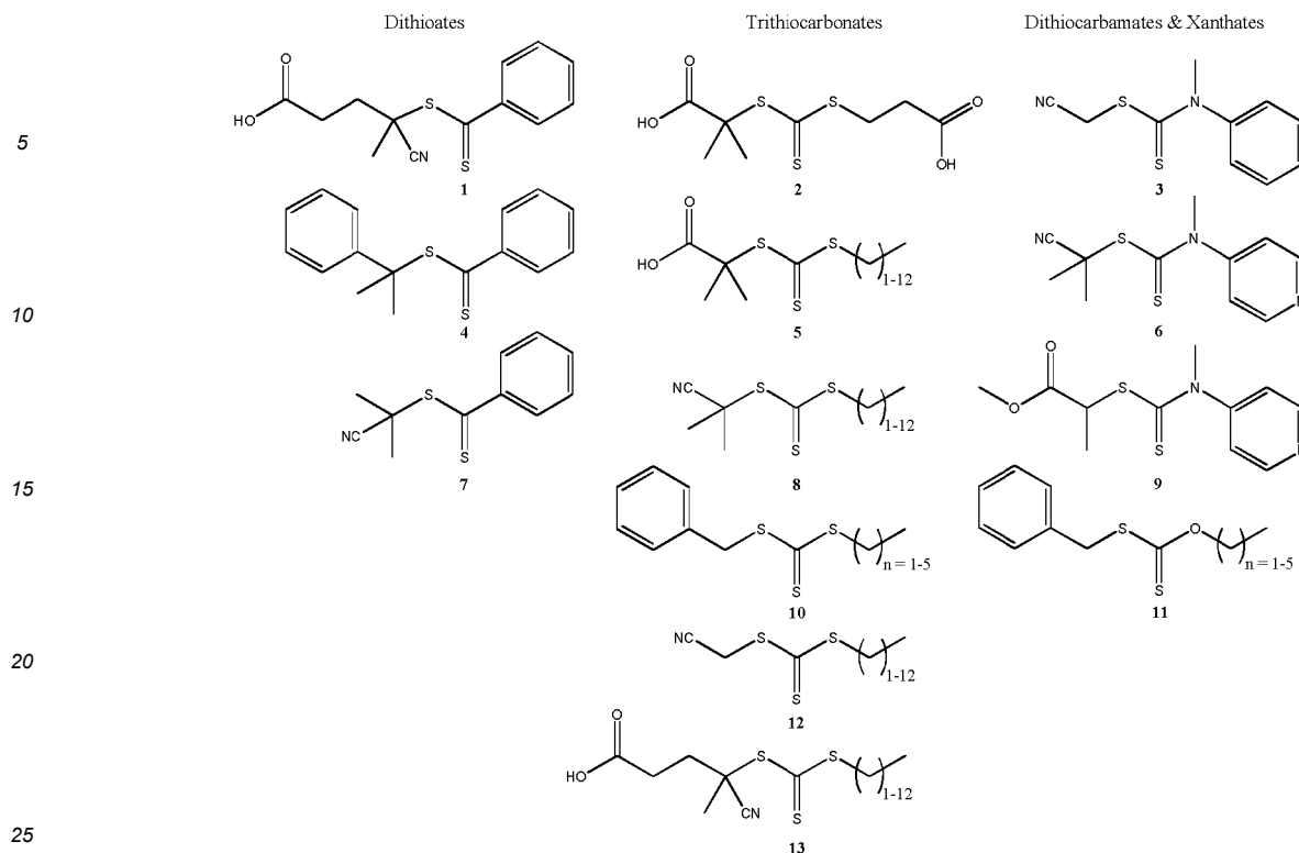
Formula VIII
