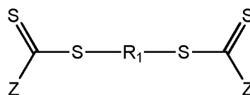
Formula VII
