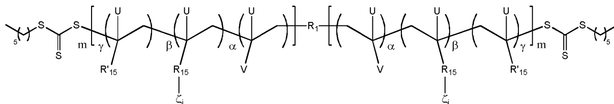
Formula VI
