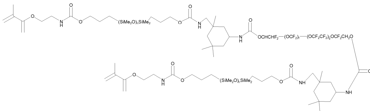
Formula XVIII
